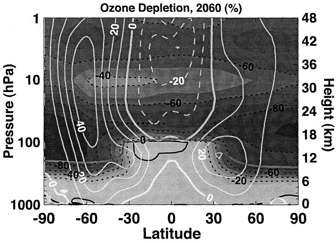
Fig. 6. Percentage total ozone difference between the WORLD AVOIDED and the reference future simulations for a decadal average (2055 to 2065). The dashed contours are in 20% increments while colors are in 10% increments. The magenta line shows the WORLD AVOIDED tropopause. The white lines show the zonal-mean zonal winds (easterlies are dashed) for the WORLD AVOIDED simulation.
