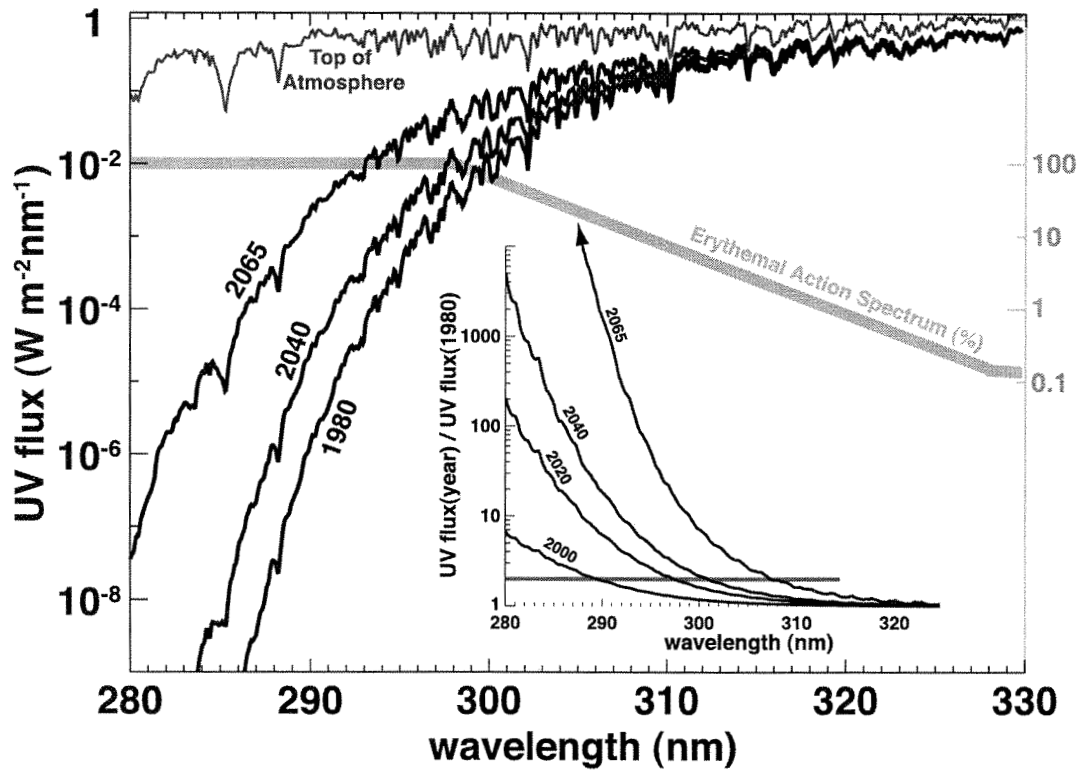
Fig. 13. UV flux ( W m^{-2} nm^{-1} ) is shown for the WORLD AVOIDED simulation in the years 1980, 2040, and 2065 (thick black lines). The UV flux is calculated using the July 30^{\circ} – 50^{\circ} N zonal-mean ozone and temperature profiles, and assuming a time of local noon on 2 July. The thick grey line shows the erythemal (sunburn) action spectrum (right hand axis). The thin darker grey line shows UV flux at the top of the atmosphere. The inset figure shows the ratio of the UV flux for the years 2000, 2020, 2040, and 2065 to its value in 1980. The horizontal grey line in this inset indicates a doubling of the flux from 1980 conditions.
