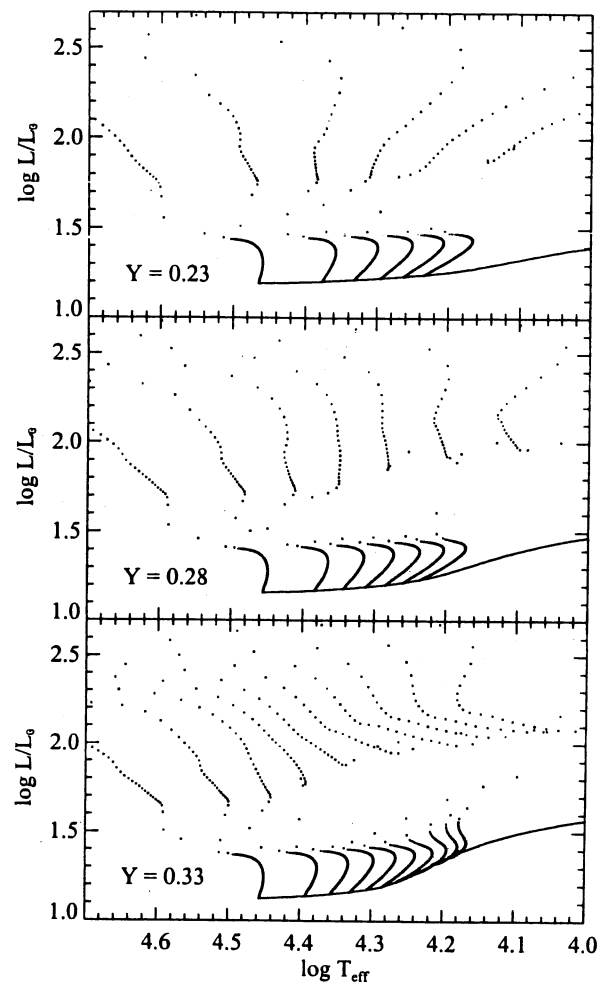
FIG. 10.— EHB and post-EHB evolutionary tracks for Z = 0.01 and Y = 0.23 (top panel), 0.28 (middle panel), and 0.33 (bottom panel). Each track is plotted by a series of points spaced every 10^6 yr during the evolution. The hottest track in each panel lies at the hot end of the EHB. The mass spacing between the tracks in each panel is 0.005 M_{\odot} . The solid curves represent the ZAHB for each composition.
