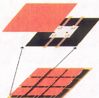
Fig 1: Conceptual layout of the 2-D array far-IR bolometer. Each pixel: 100 x100 \mu m.
