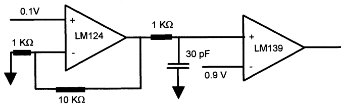
Fig. 9. Application for which negative SETs with amplitudes greater than -0.2 V and longer than 5 ms
