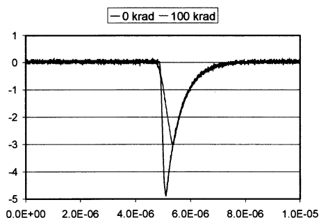
LM139 Voltage Comparator
