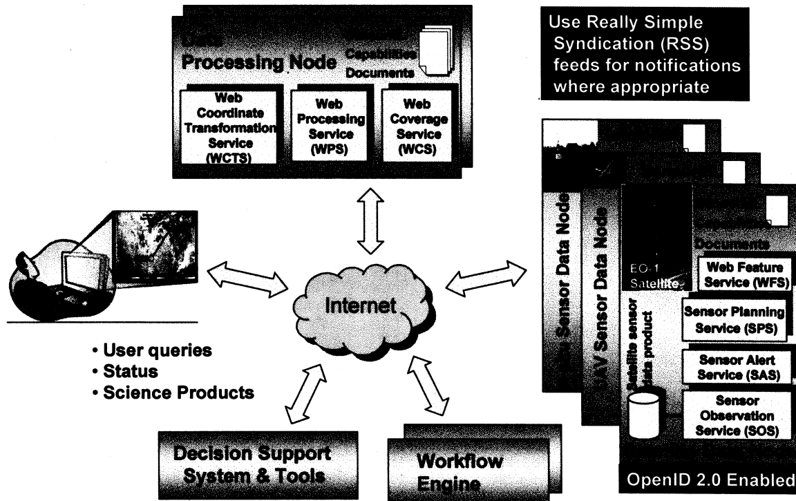
Figure 1 User-centric sensor web reference architecture
