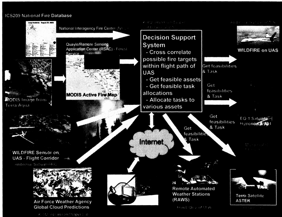
Figure 3 Composite sensor web demonstration
