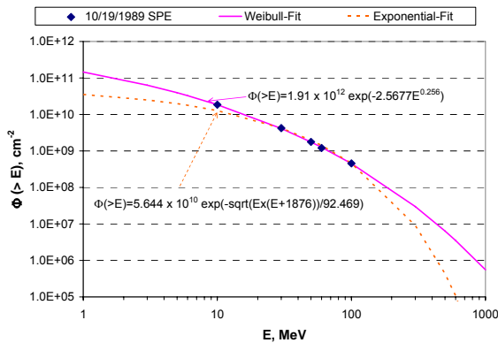
Figure 4. Fit to proton fluence measurements for continuous energy spectrum of October 19, 1989 SPE.
