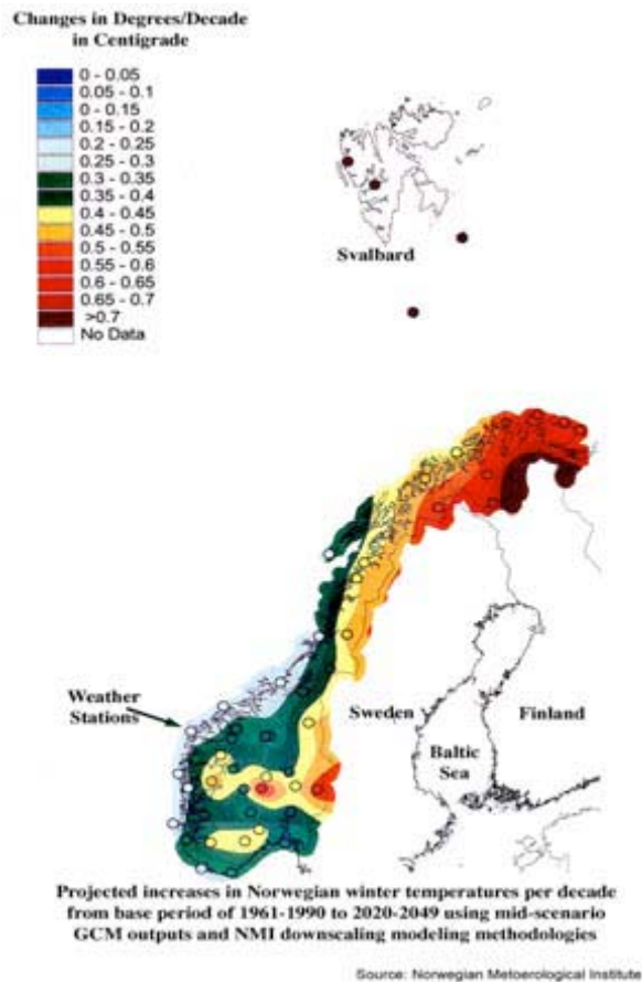
Figure 2. Future warming in Norway showing increased future temperatures in the north and east in region important for reindeer grazing in winter.
