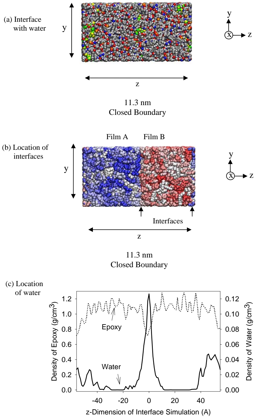
Figure 4. (a) Molecular structure of epoxy interface with water, (b) location of interfaces, and (c) location of water at interfaces along the z-direction. Colors as in Figures 2 and 3 with the water hydrogens in green and oxygens in yellow.
