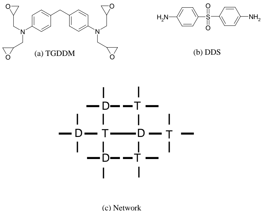
Figure 1. Molecular structures of (a) TGDDM and (b) DDS and (c) the network that is formed by crosslinking them. T=TGDDM; D=DDS.
