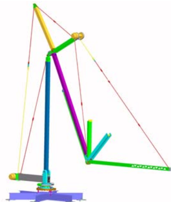
Figure 3. Tension Members Lifted Off s3a and s3b with LSMS in Fork-Lift
