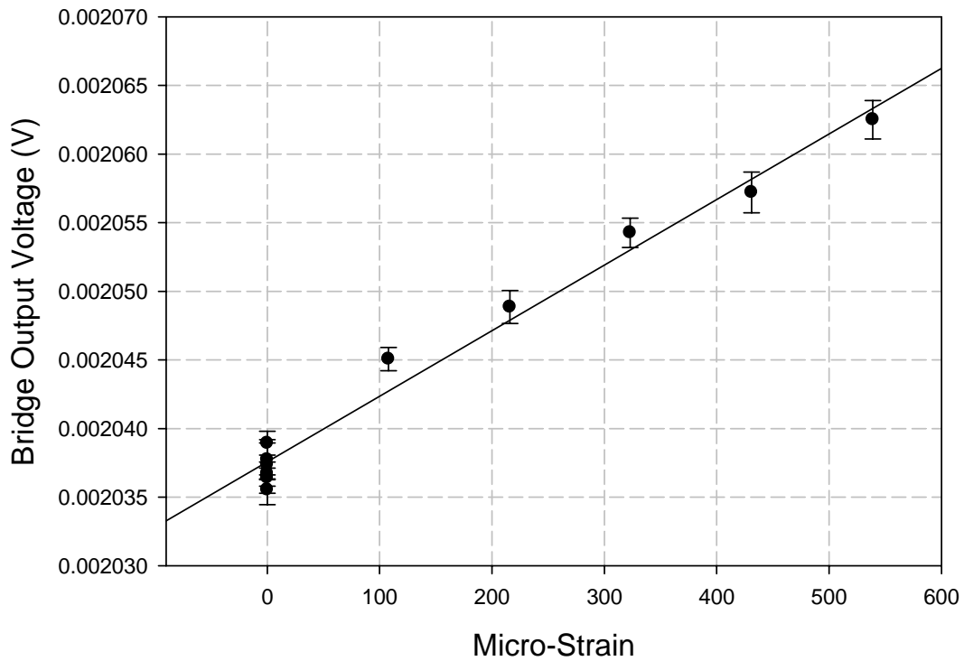
Figure 6a: Response of CNT yarn bridge output voltage of the test beam
