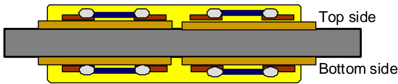
Cross sectional view of the SS test beam
