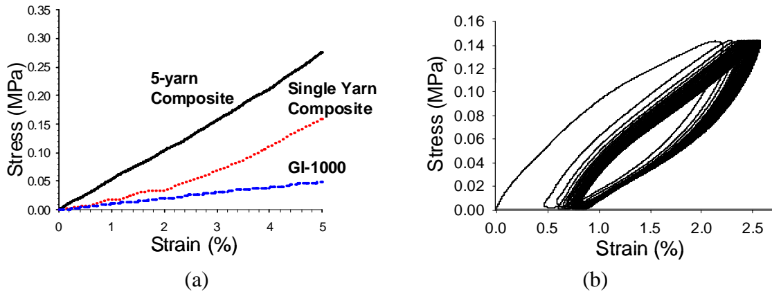
Figure 3: Figure 3a shows Engineering Stress-Strain response of the 5-yarn composite dog bone shape specimen, that of single yarn and the GI-1000 silicone rubber. Figure 3b shows the dynamic mechanical analysis tests of 50 cycles of a 5-yarn with GI-1000 specimen.
