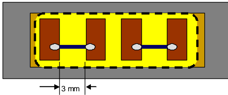
Figure 5a: This figure shows part of the cross sectional and top views of the test beam. Top view shows only two yarns (half view).
