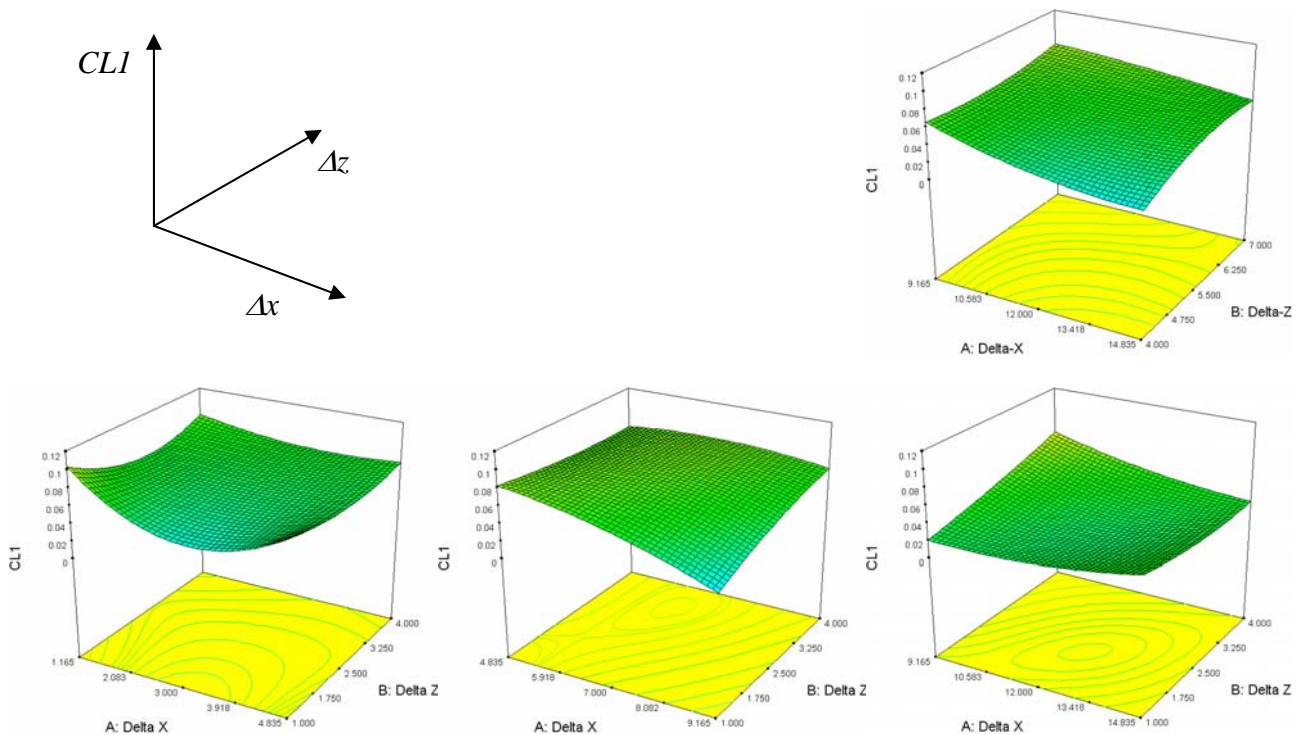
Fig. 17. Composite plot of booster model lift coefficient response surfaces in subspaces 1', 2', 4', and 5'; spherical CCD; \Delta \alpha = 2.5 degrees.
