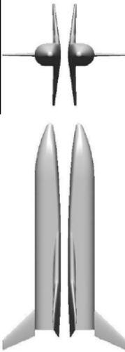
Fig. 2. LGBB bimese wing-body configuration in belly-to-belly arrangement.
