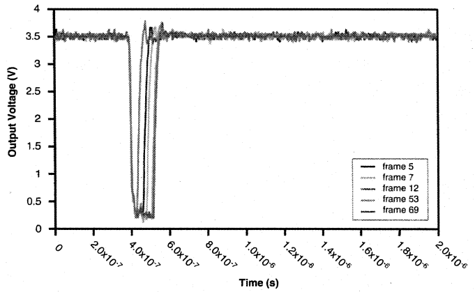
Fig. 2. HCPL625K Typical SET waveform when optocoupler is on.
