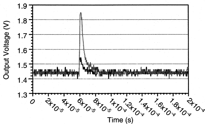
Fig. 5. SAT8605R typical SET.
