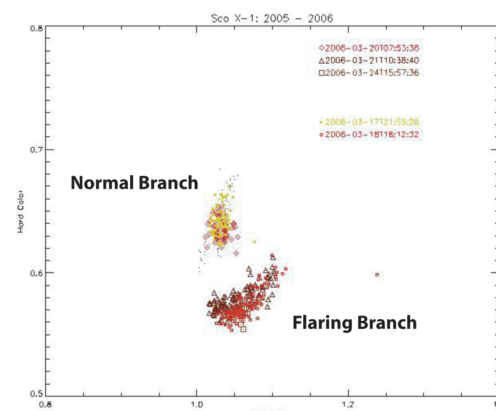
Figure 3: A Sco X-1 X-ray color-color diagram derived from RXTE/PCA data. The data were chosen to due to there temporal overlaps with the INTEGRAL observations.
