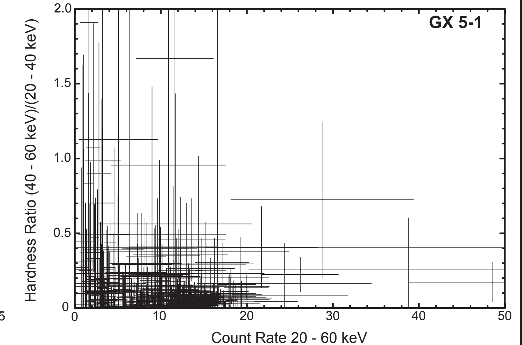
Figure 6: Color-Intensity diagram for GX 5-1 from IBIS/ISGRI data. Each data point represents 2 hours of data.
