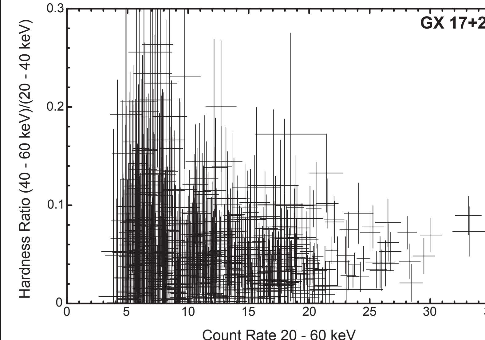
Figure 5: Color-Intensity diagram for GX 17+2 from IBIS/ISGRI data. Each data point represents 2 hours of data.
