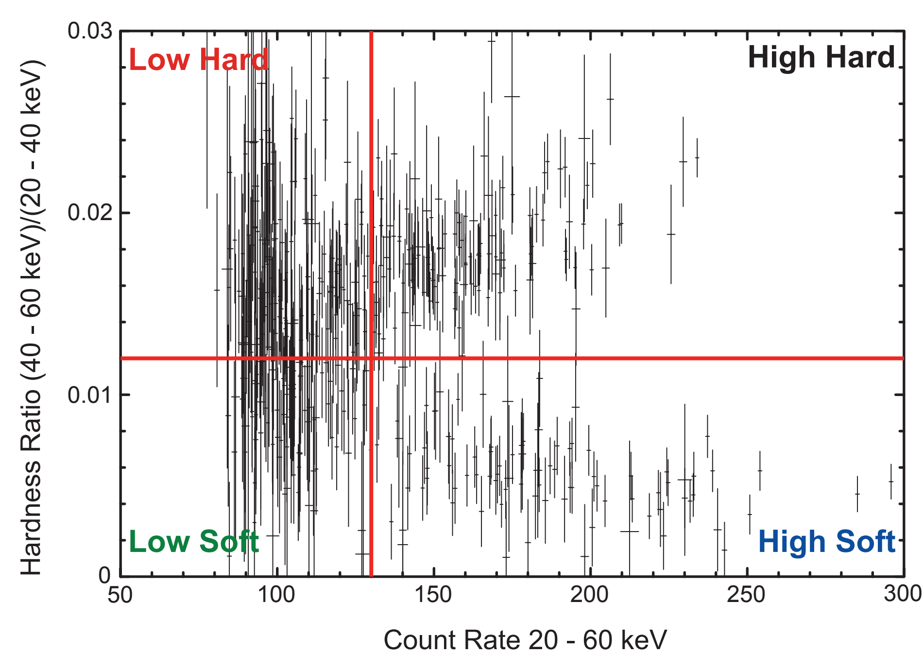
Figure 1: Color-Intensity diagram for Sco X-1 from IBIS/ISGRI data. Each data point represents 2 hours of data. The diagram shows distinct hard and soft spectral states.
