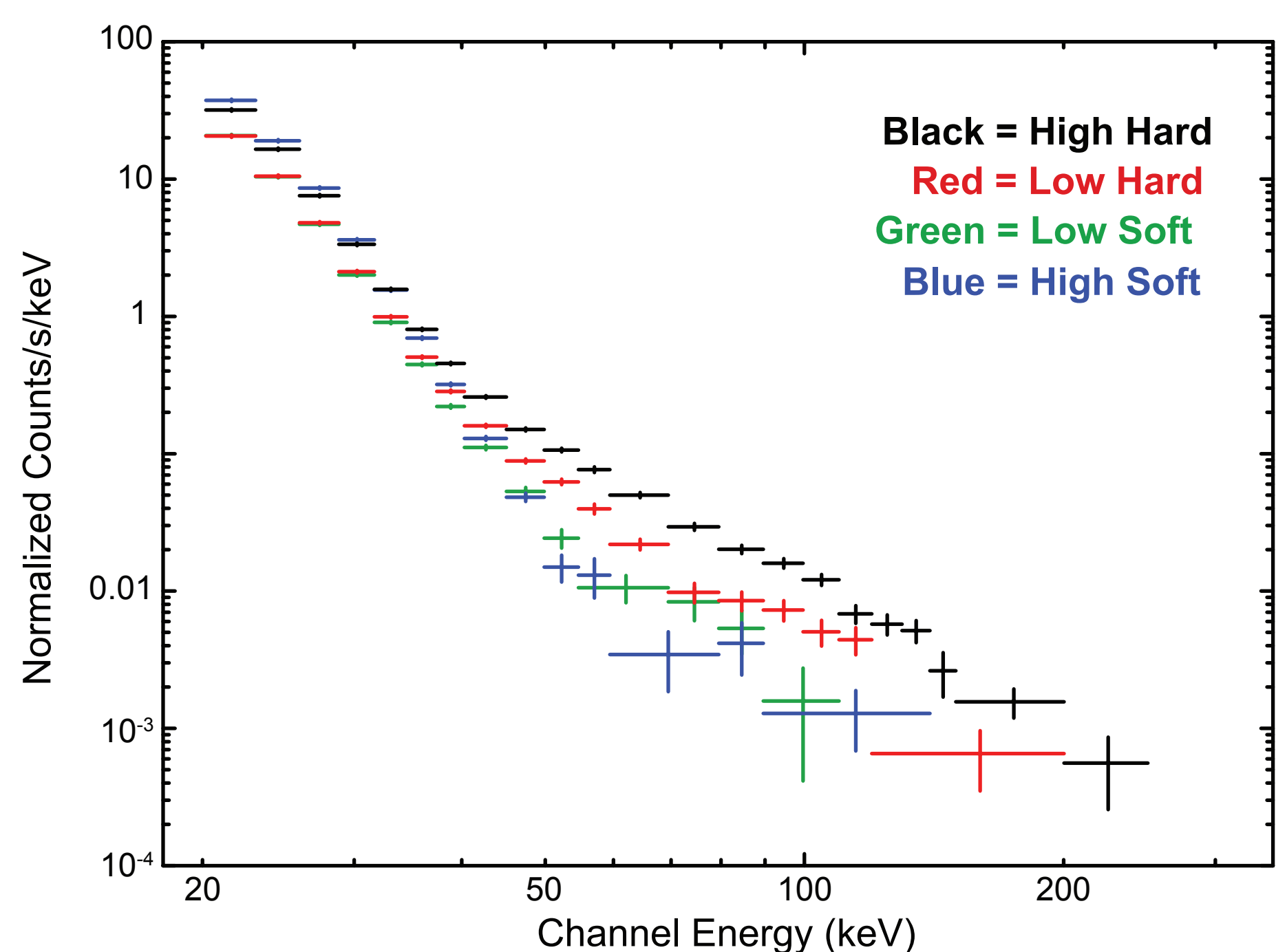
Figure 2: Count spectra for the 4 states illustrated in Figure 1.
