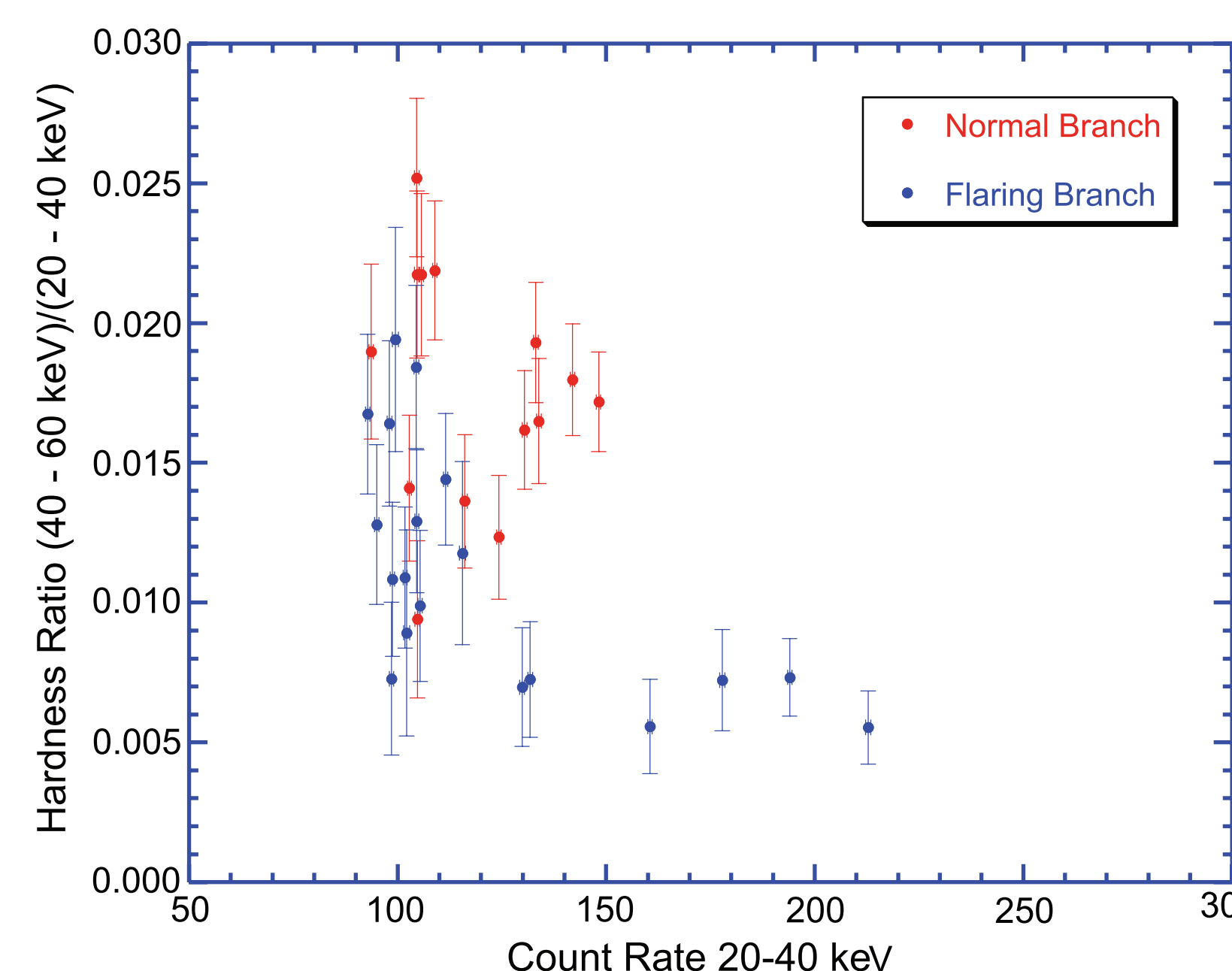
Figure 4: Color-Intensity diagram for Sco X-1 using the subset of the data in Figure 1 which fell within \pm 6 hours of a RXTE/PCA observation shown in Figure 3.
