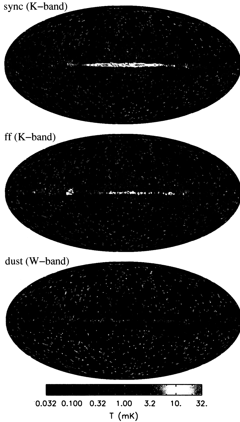
Fig. 7.— Temperature maps for foreground components as determined by the MCMC fitting process for the “base” model. Maps from other models are qualitatively similar. Synchrotron and free-free temperatures are as measured at K-band, dust is measured at W-band. Gray pixels are those masked due to point sources or flagged as problematic. Top – synchrotron; middle – free-free; bottom – dust
