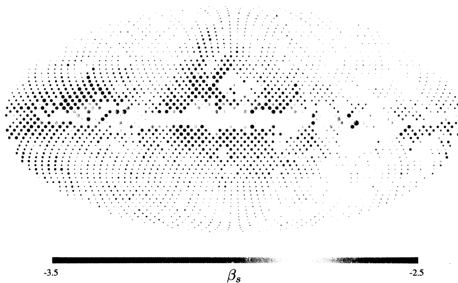
Fig. 11.— Map of synchrotron spectral index for the “base” fit, binned to N_{\text{side}} = 16 . Color shows the value of the spectral index, and circle area indicates the weight \sigma_\beta^{-2} given by the fit. Pixels with \chi_\nu^2 > 2 were explicitly de-weighted.
