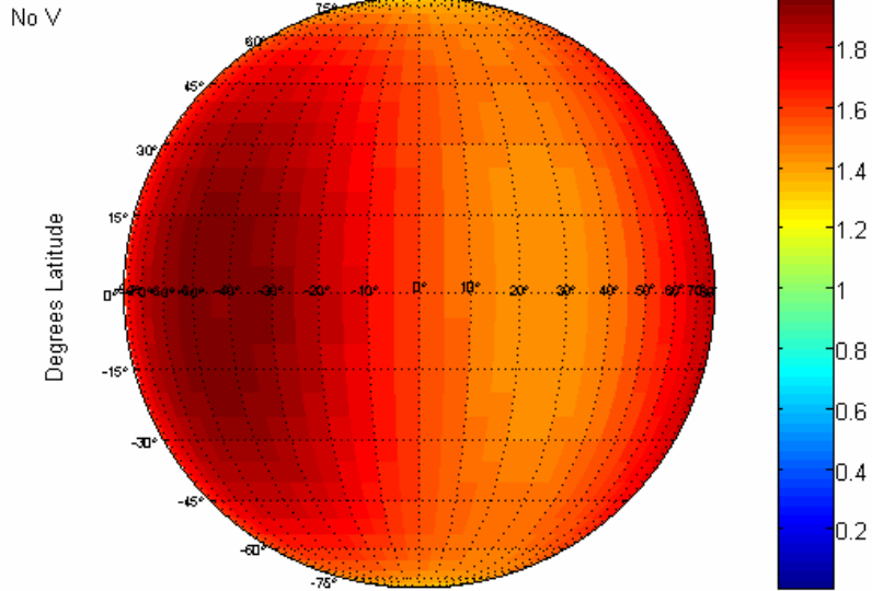
1 State 10/27/06 22:59 pm .31 Phase Evening Observation
