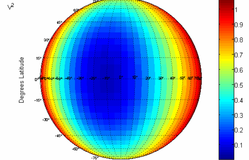
1 State 6/20/06 03:50 am .30 Phase Morning Observation
