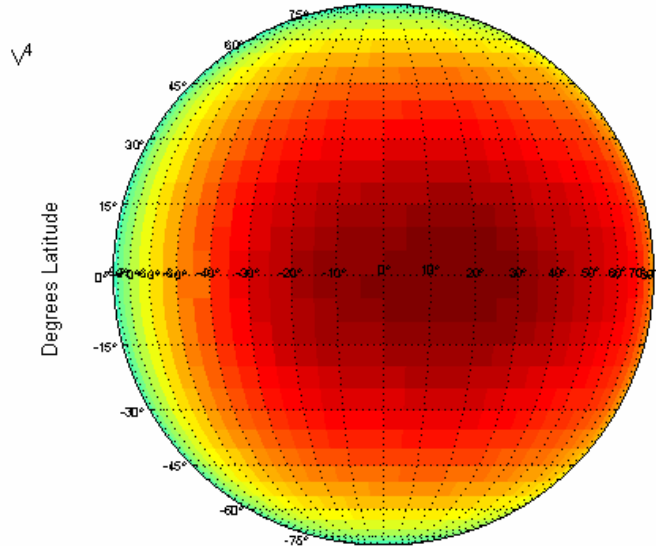
Flux Impacting on Near Side of Lunar Surface (in selenographic coordinates)
