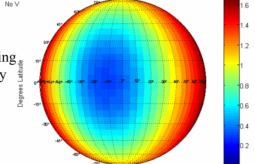
Flux Impacting on Near Side of Lunar Surface (in selenographic coordinates)
