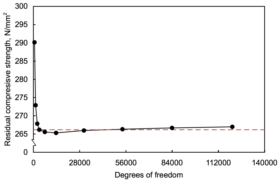
Figure 8. Effect of mesh density on computed residual strength
