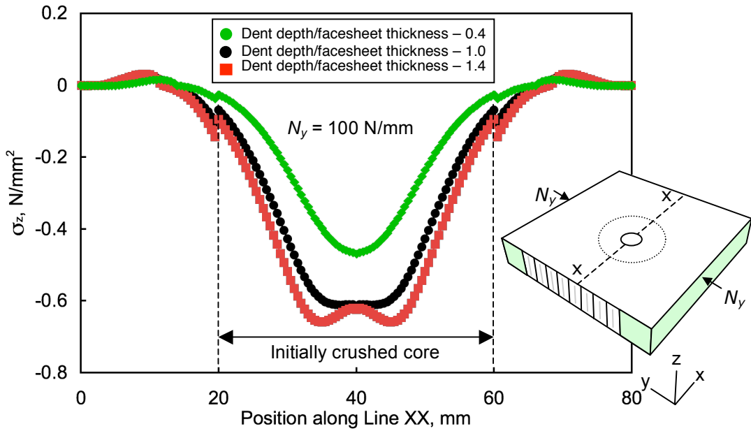
Figure 13. Effect of dent depth on thickness-direction core stresses along Line XX
