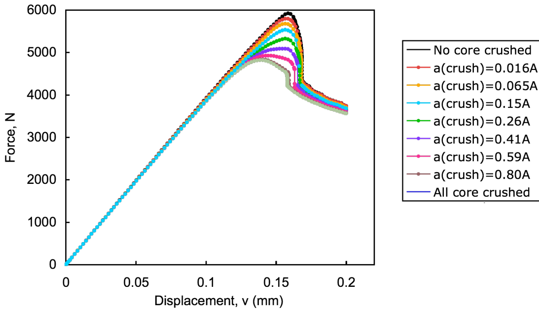
Figure 14. Effect of core crush region size on force-displacement response
