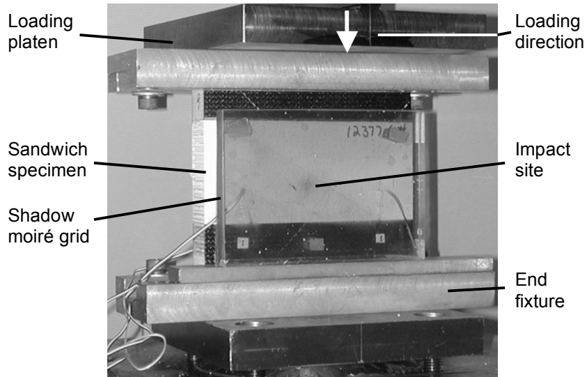
Figure 1. Test configuration of axial compressive test on a sandwich specimen
