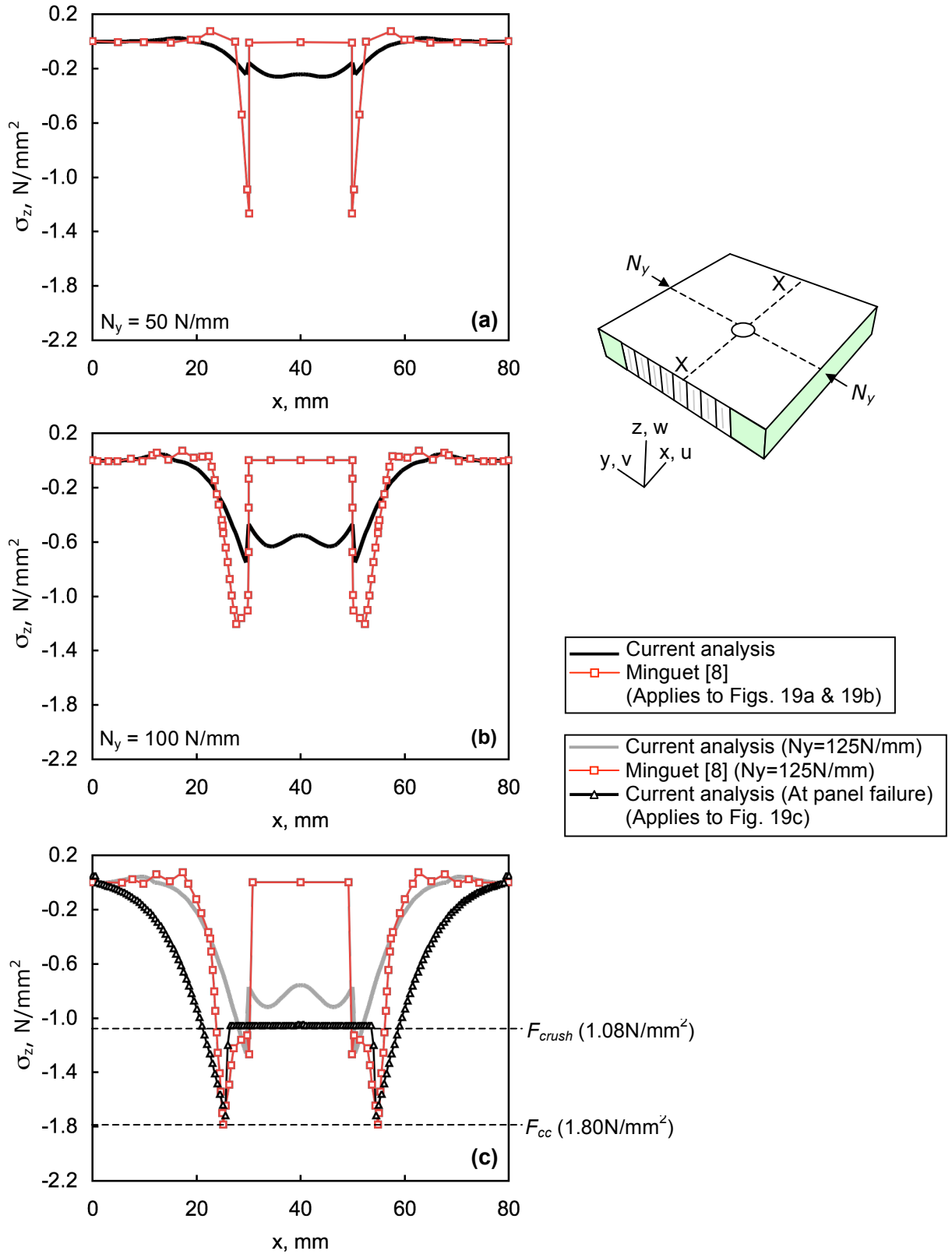
Figure 19. Thickness-direction core stresses along Line XX at various values of N_y
