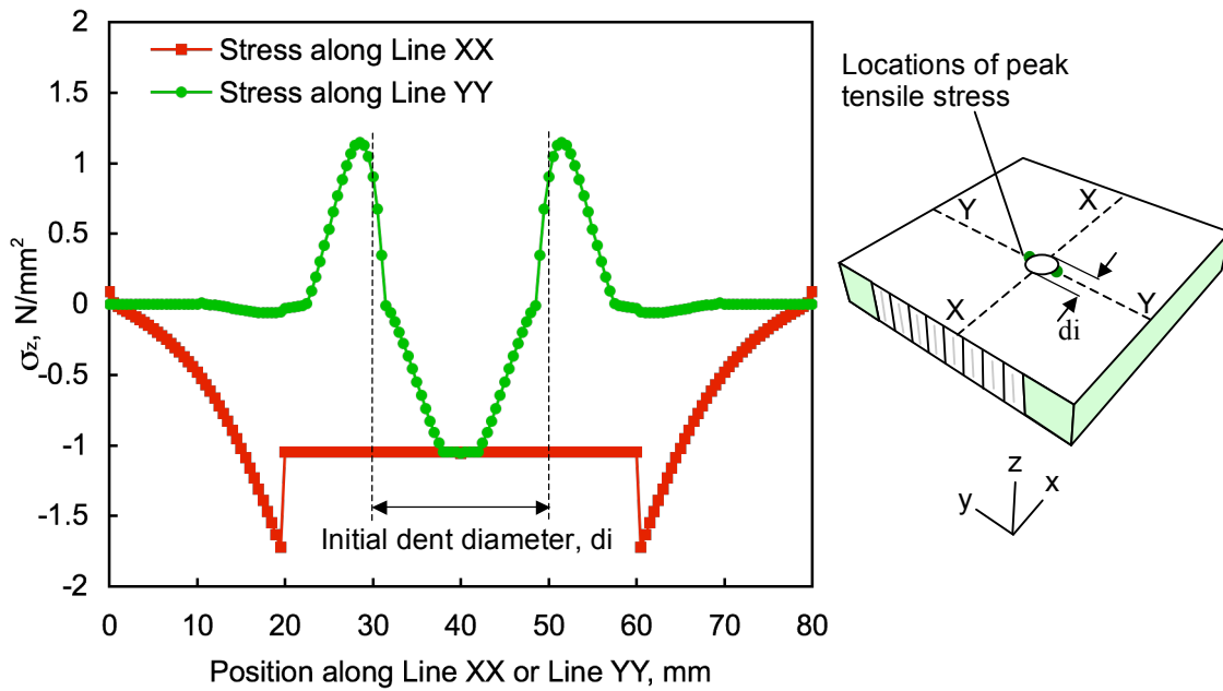
Figure 15. Thickness-direction core stresses along Lines XX and YY
