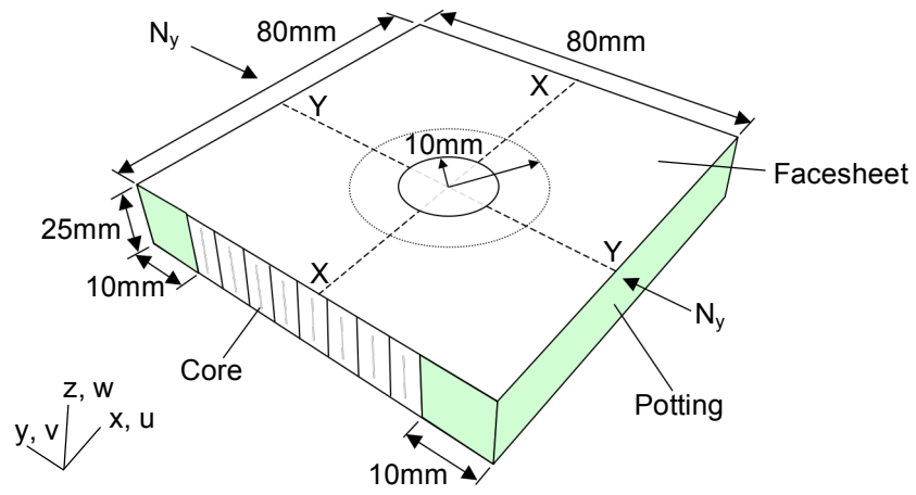
Figure 10. Schematic of sandwich specimen modeled in parametric studies
