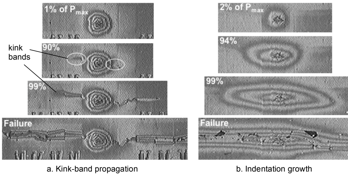
Figure 2. Examples of compressive failure modes ( P_{max} denotes force at panel failure)
