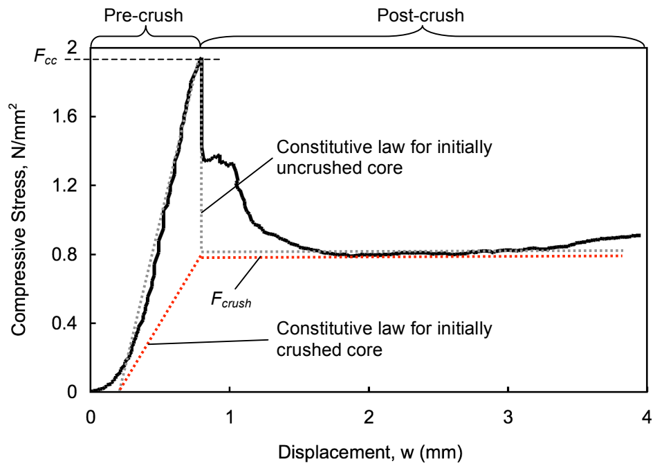
Figure 6. Measured and idealized core crush behavior
