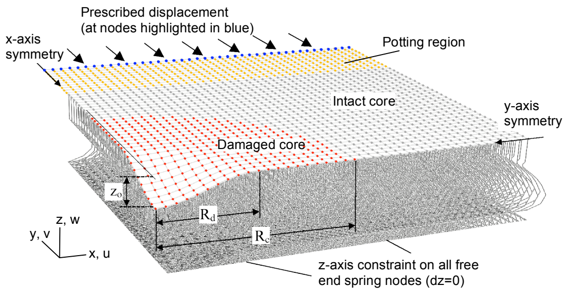
Figure 4. Finite element mesh used to model sandwich panel
