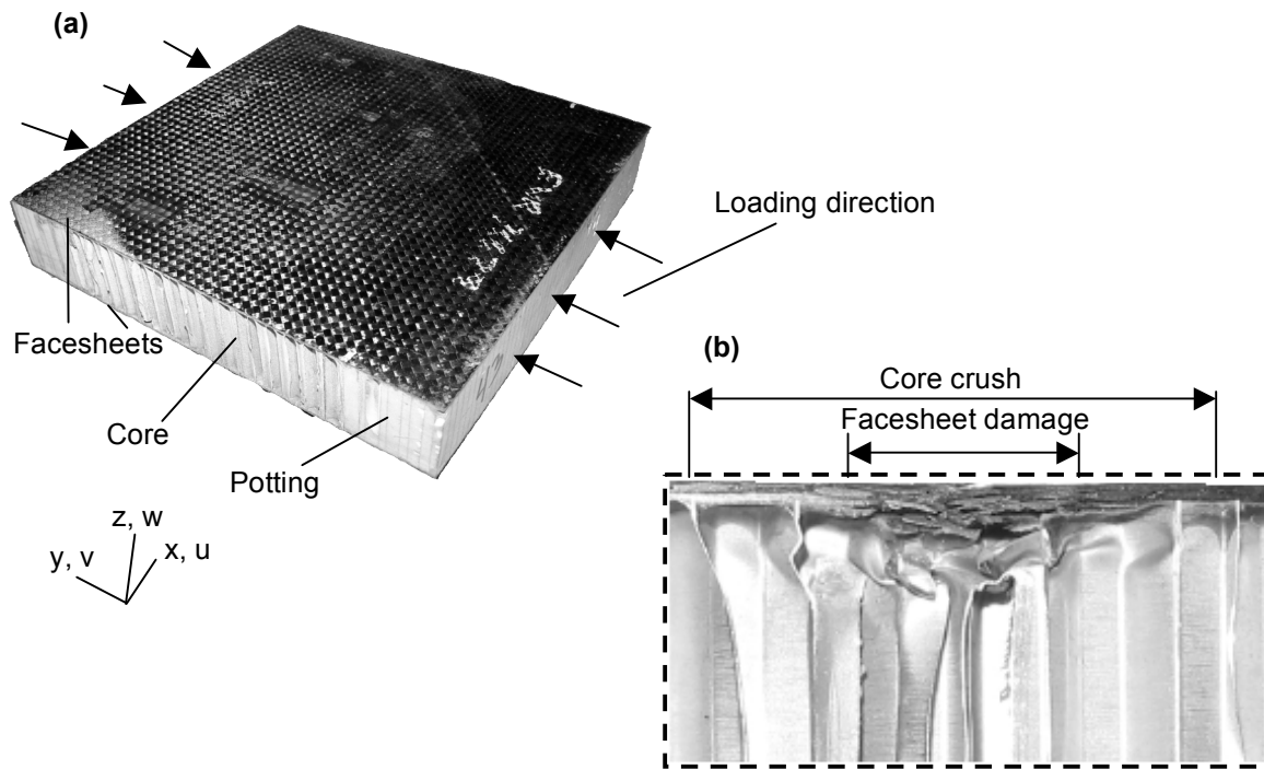
Figure 3. Impact-damaged sandwich panel and core crush resulting from impact
