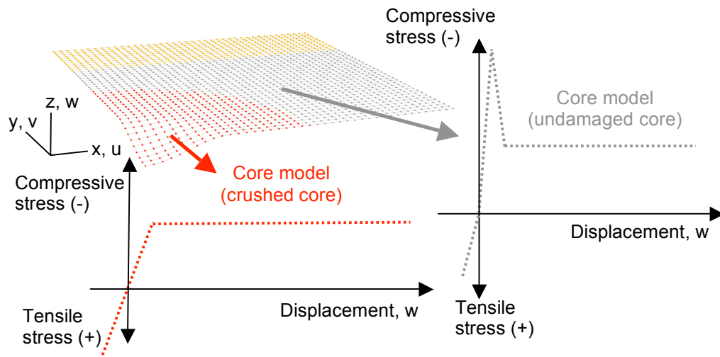
Figure 7. Summary of assignment of core constitutive models
