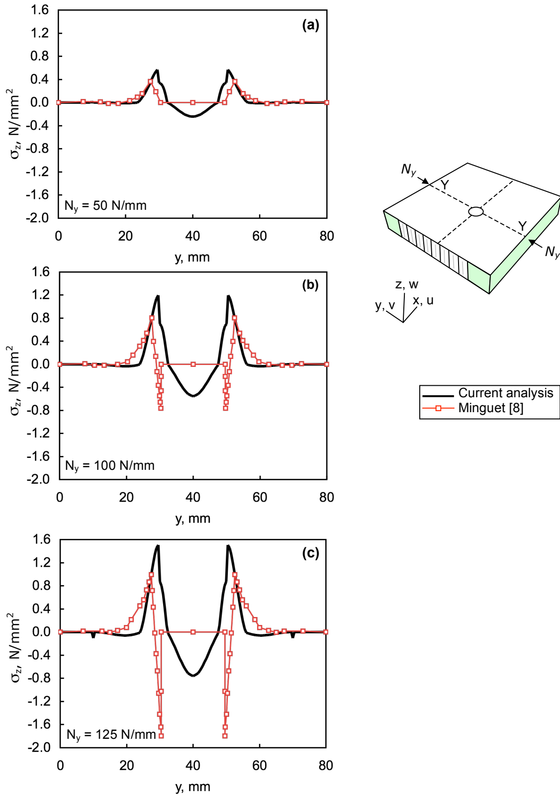
Figure 18. Thickness-direction core stresses along Line YY at various values of N_y
