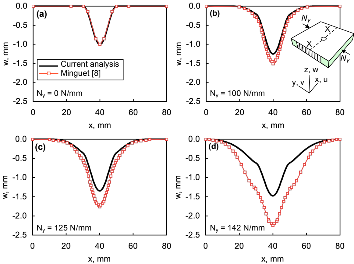
Figure 17. Transverse displacement along Line XX at various values of N_y
