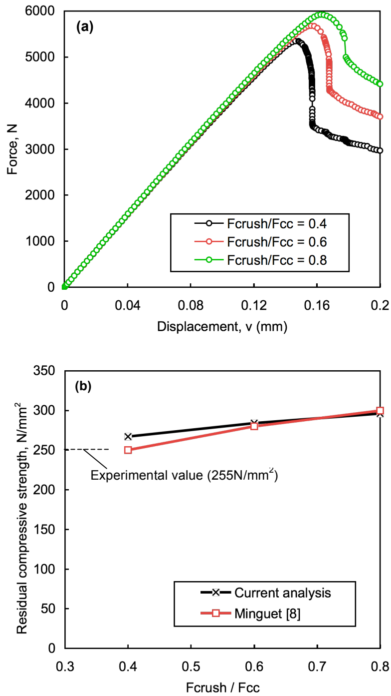
Figure 21. Effect of core crush ratio, F_{crush}/F_{cc} on force-displacement response and strength
