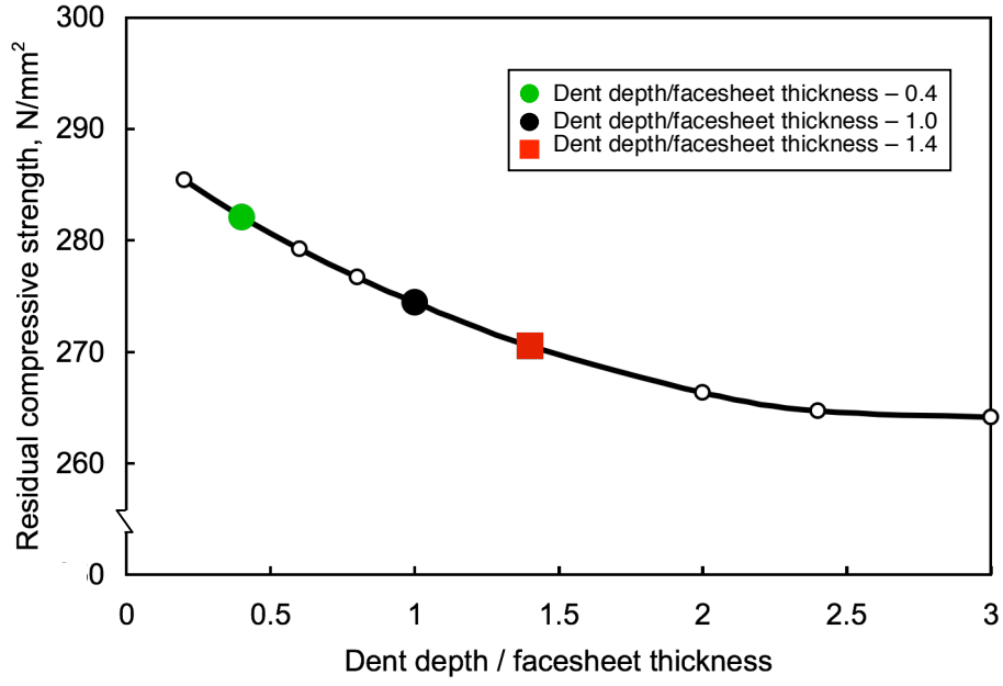
Figure 12. Effect of dent depth on computed residual strength
