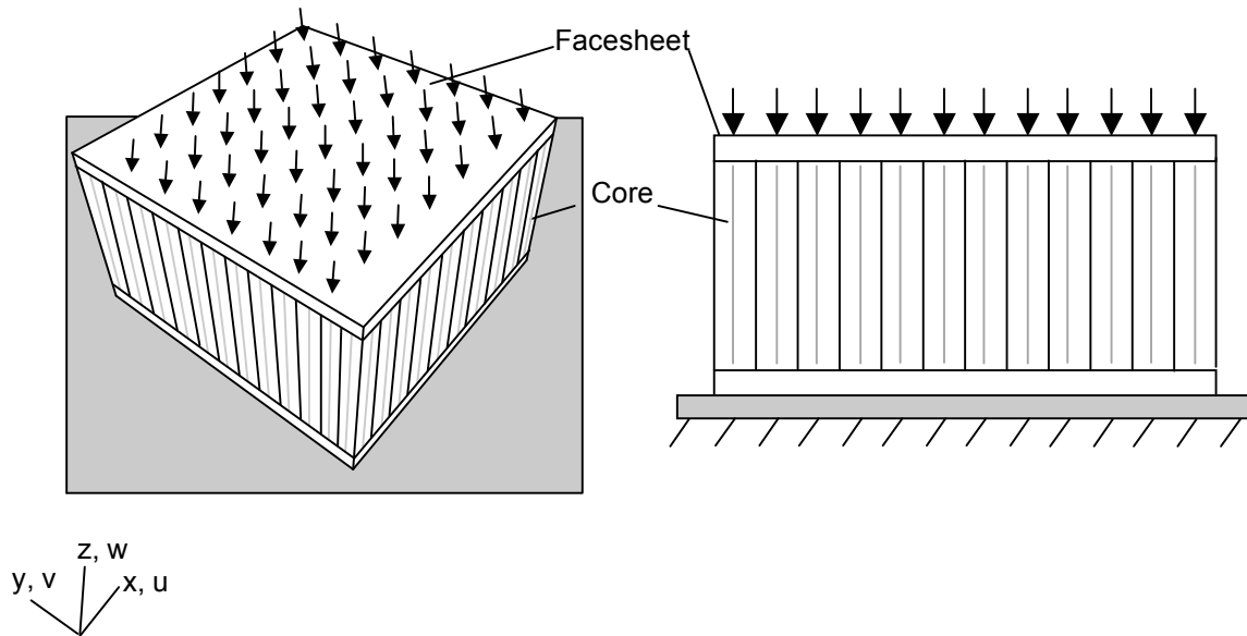
Figure 5. Flatwise compression specimen for characterizing core crush behavior
