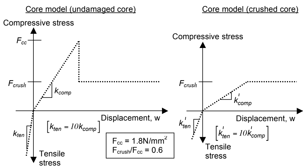
Figure 11. Core constitutive models used in parametric studies
