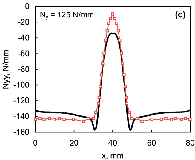
Figure 20. Distribution of in-plane reaction forces in facesheet along Line XX
