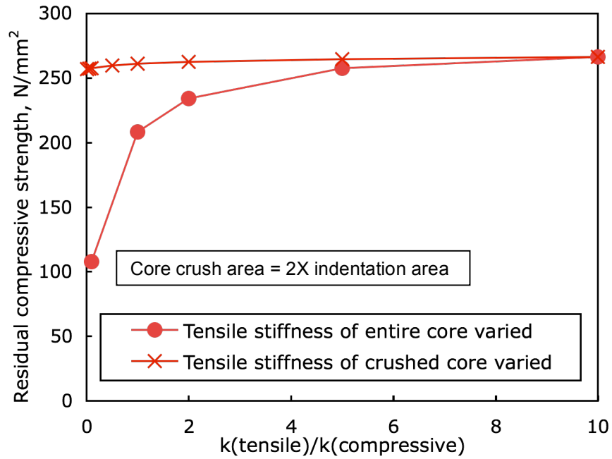
Figure 16. Effect of core tensile stiffness on computed residual strength
