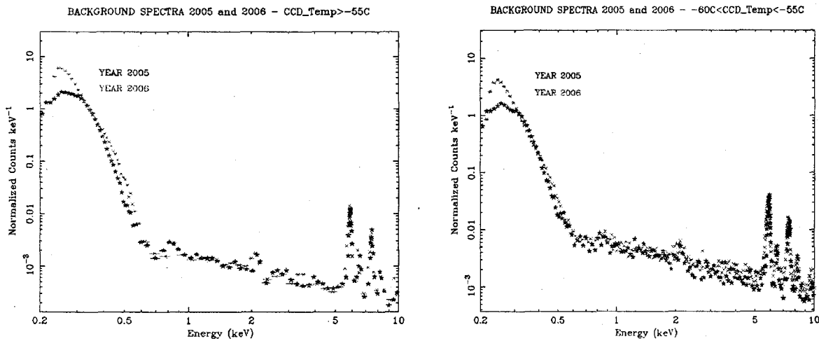
Fig. 2. Background spectra from year 2005 and year 2006 extracted at CCD temperature ranges of T > -55C and -60C < T < -55C . The spectra have been extracted by selecting event grades 0 to 12 only. For both temperature ranges, the comparison of the spectra shows an increase of low energy background events during 2006 compared to 2005.
