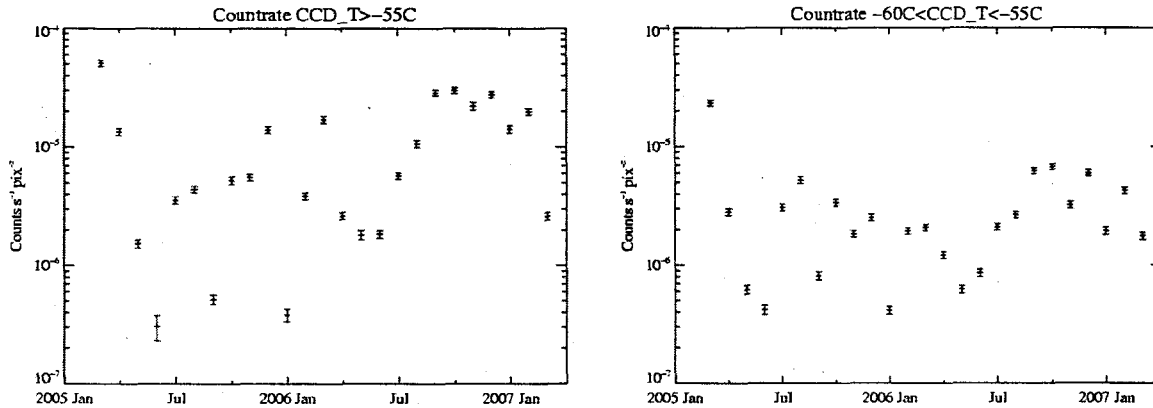
Fig. 1. Background count rate since the start of the mission at CCD temperatures -60C < T < -55C and T > -55C . The count rate increases with temperature but there is no evidence of strong evolution since the start of the Swift mission.
