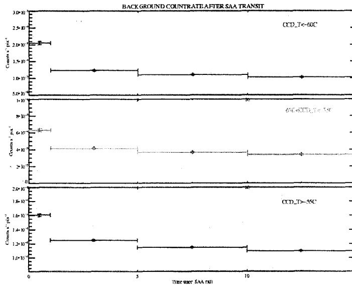
Fig. 4. The background count rate evaluated at increasing time intervals after the exit time of the SAA passes. The count rate is higher just after the SAA transit, and it levels off at later times.
