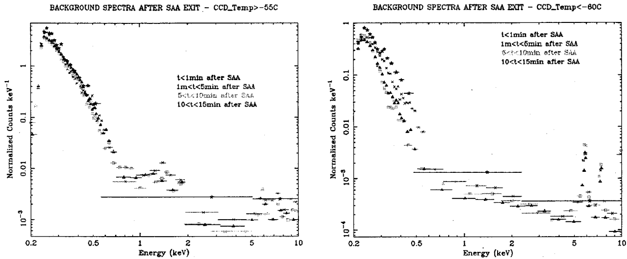
Fig. 5. The background spectra extracted at increasing time intervals after the exit time of the SAA passes.
