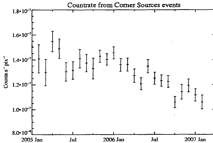
Fig. 3. The count rate of the events from the spectral line at 5.9keV has decreased since the start of the mission. These events are produced by k- \alpha and k- \beta emission of the ^{55}\text{Fe} radioactive corner sources with a half-life of 2.7 years.
