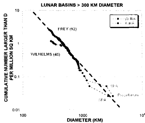
Figure 3. Cumulative frequency curves for impact basins \geq 300 km diameter from Wilhelm's [9] based on traditional photogeologic mapping (red) and our mapping based on the ULCN topography (blue). The curves are very similar from 1200 km down to about 500 km diameter, but at smaller diameters Wilhelm's inventory has far fewer features than we find in the topography. Dashed line is a -2 power law.
