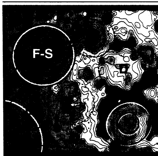
Figure 1. Portion of the lunar farside at 10N, 172W. Color is stretched ULCN topography. Contour interval 400 m. Basins identified by Wilhelms [10] shown as white circles: K=Korolev (440 km) and F-S = Freundlich-Sharonov (600 km). These have strong expression in the topography (solid black circles). The diameter suggested by the topography is in good agreement with Wilhelms' diameters, though F-S may have more rings than he suggested. Basins \geq 300 km diameter not recognized by Wilhelms but suggested by topography (dashed black circles) include several Korolev-size features (at D) and a less obvious feature at P.
