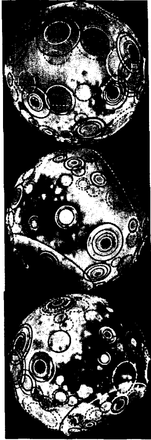
Figure 2. Equatorial views of the ULCN topography at three longitudes (0, 120 and 240W). Blues = lows, reds = highs. Wilhelm's basins \geq 300 km shown as white circles. His "Probable or possible basins" shown as thinner white lines. Black circles show our mapping of Wilhelm's basins derived from ULCN topography, which sometimes suggests different ring assignments and reveals the existence of many basins not previously recognized by photogeologic mapping (dashed black circles). We find at least 92 large basins compared with the 45 listed in [10].
