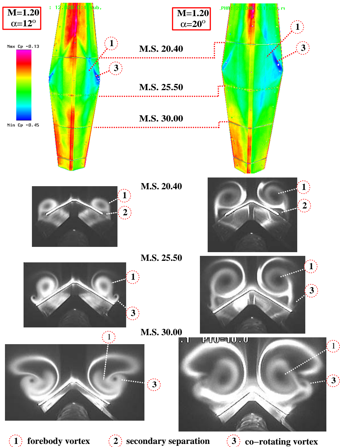
Fig. 14. Comparison of PSP and LVS images on the faceted missile model at \alpha = 12^\circ and \alpha = 20^\circ , M = 1.20
