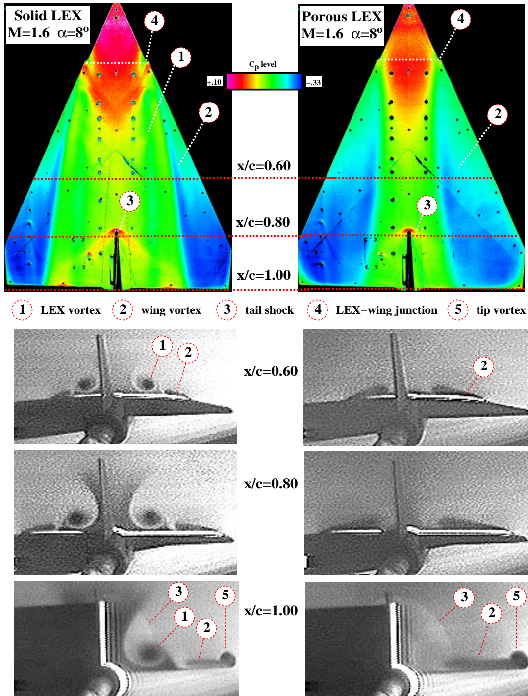
Fig. 7. Comparison of PSP and LVS images on the 65-degree cropped delta wing model with solid LEX and porous LEX at M = 1.6 , \alpha = 8^\circ
