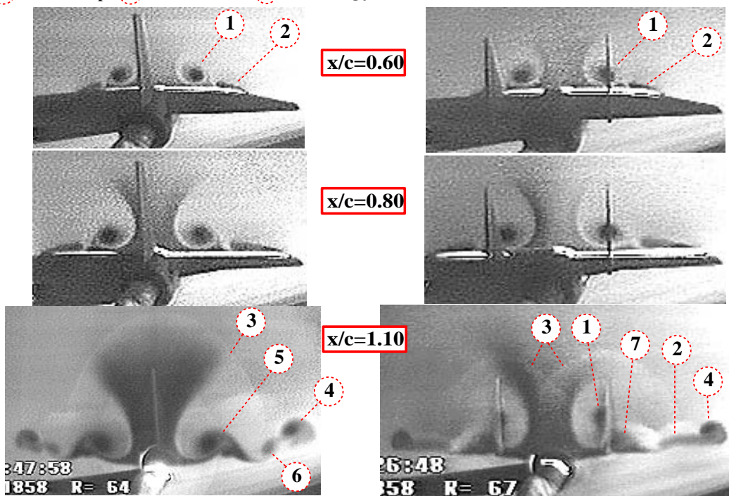
Fig. 10. Comparison of PSP and LVS images on the 65-degree cropped delta wing model with solid LEX and centerline and twin vertical tails at M = 1.6 , \alpha = 8^\circ
