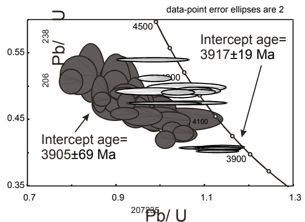
Figure 2. Common Pb uncorrected U-Pb analyses of apatite grains from the samples 14306 (dark grey) and 14066 (light grey). Zircon data from both samples (white) are shown for comparison.
