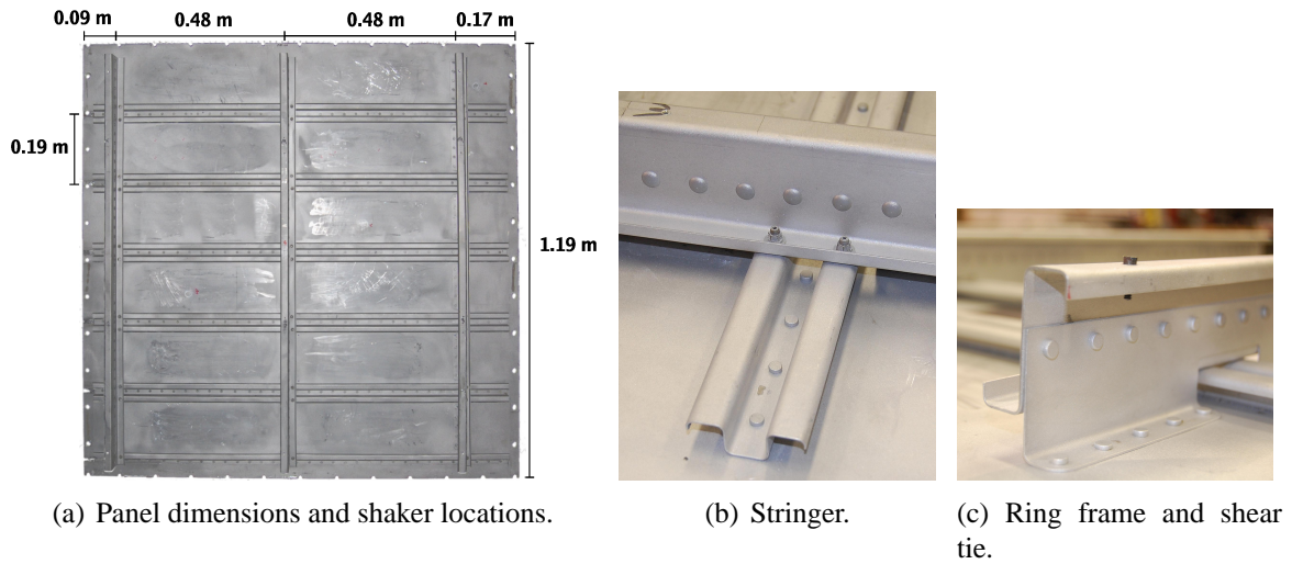
Figure 2: Test structure.
