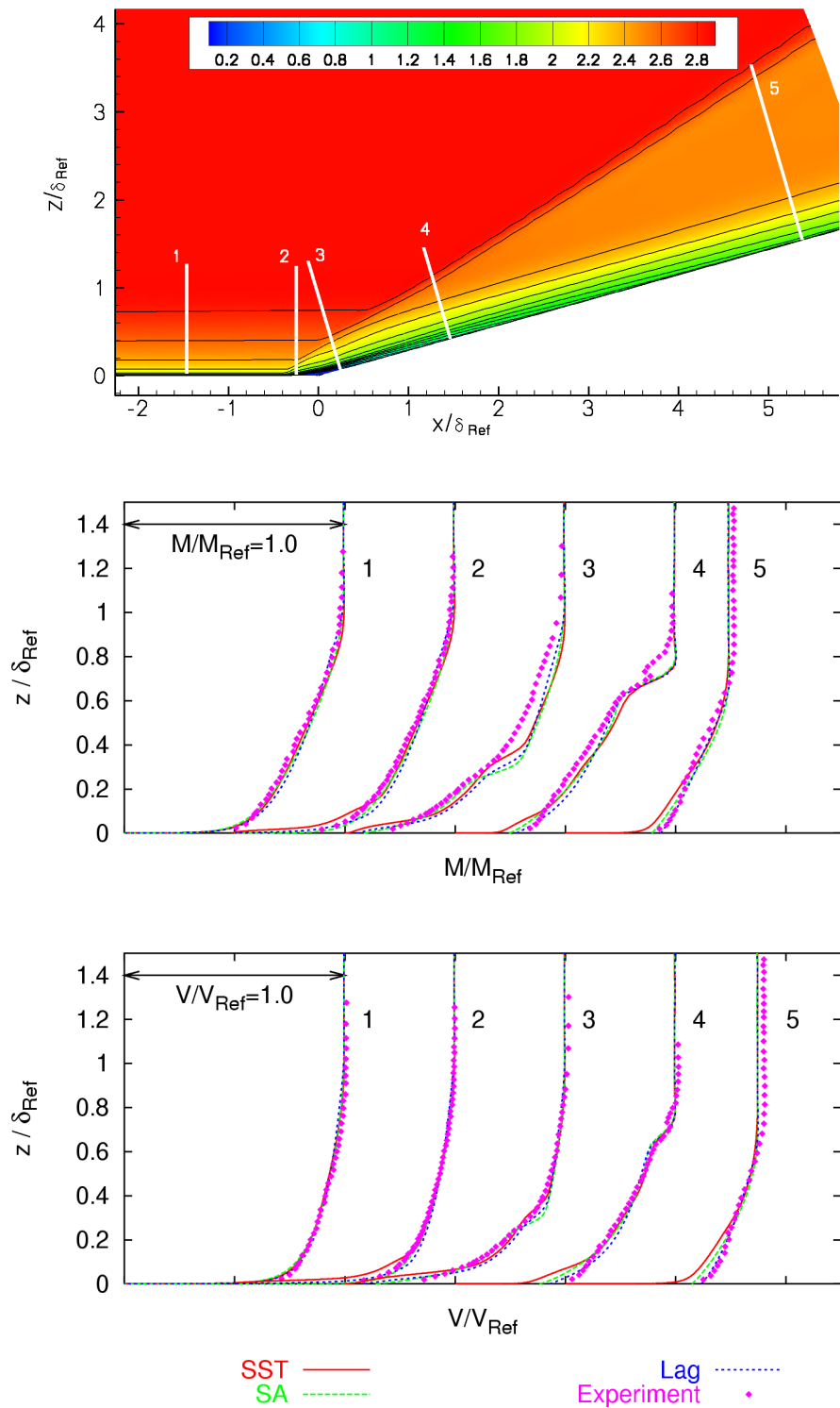
Figure 8. 16^\circ ramp: (a) Mach contours with profile locations indicated. (b) Mach profiles. (c) Velocity profiles.
