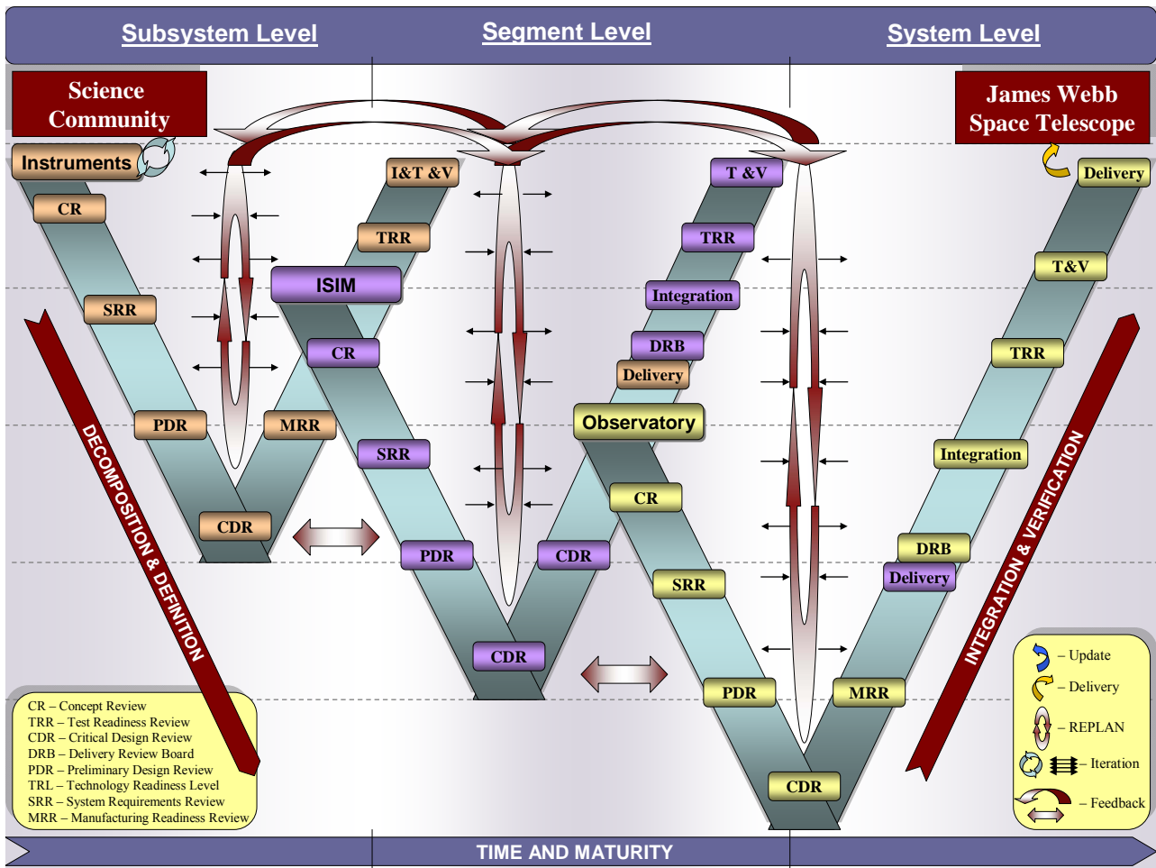
Figure 3. Schematic representation of systems engineering process used on JWST/ISIM. [1],[2]
