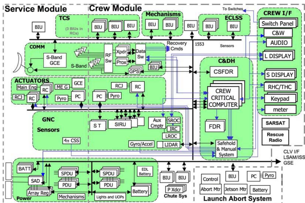
Figure 5.3-14. Notional Example of a Box Level Block Diagram
