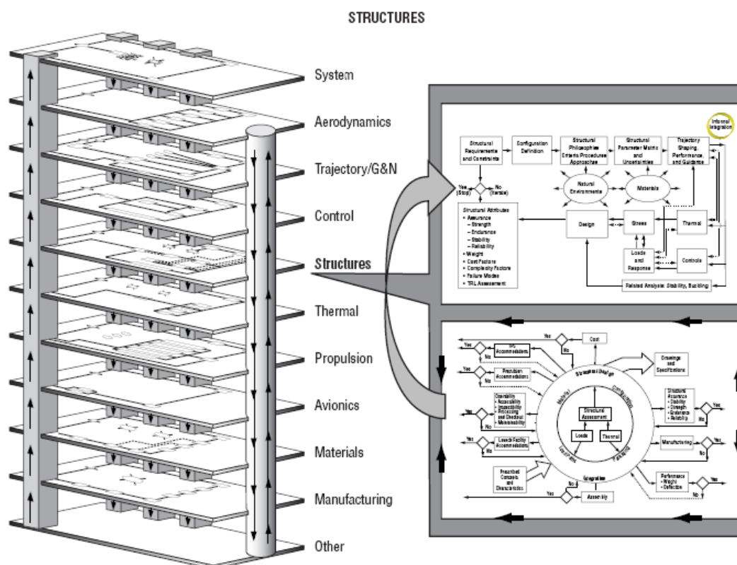
Figure 4.3-1. Design Process Technical Integration – Structure Design Function [ref. 9]
