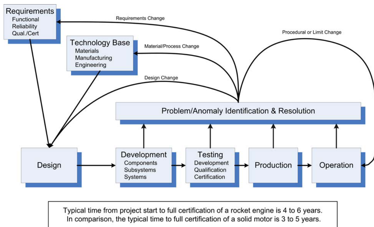
Figure 8.3-1. Propulsion System Development Process
