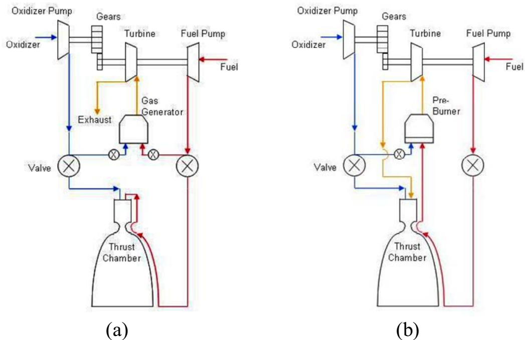
Figure 8.5-4. Gas Generator Cycle (a), and Staged Combustion Cycle (b)
