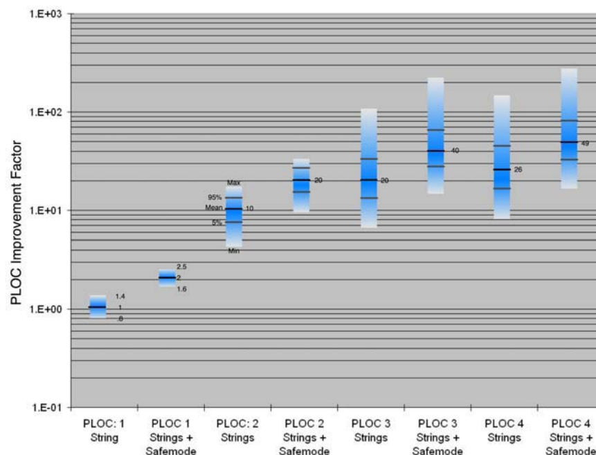
Figure 5.3-7. Example Comparison of Alternatives vs. Probability of Loss of Crew Including Uncertainty [ref. 4]
