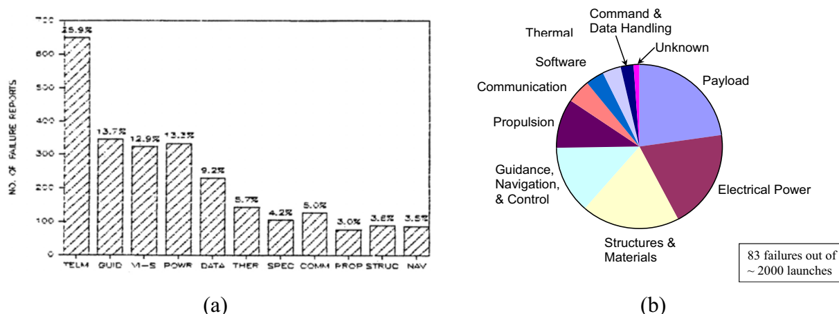
Figure 5.2-5. Distribution of Failures by Subsystems [refs. 1, 17]
