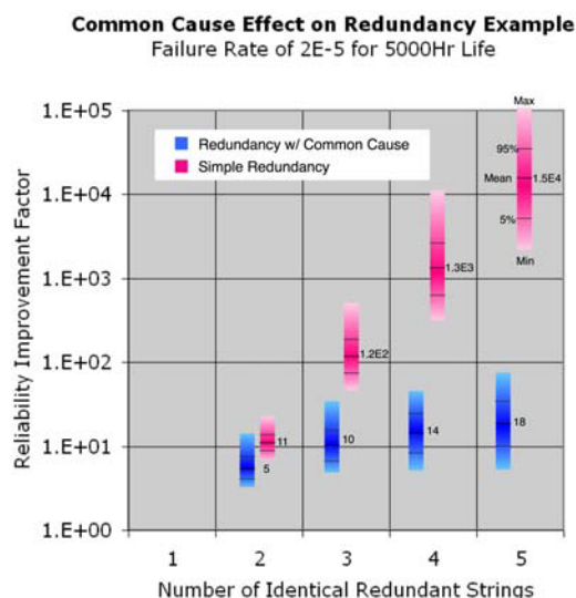
Figure 5.3-12. Common Cause Effect on Redundancy [ref. 4]
