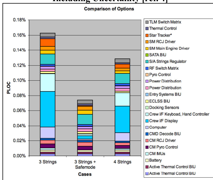
Figure 5.3-8. Example Comparison of Electrical Systems Element Contribution to PLOC [ref. 4]
