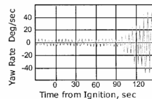
The first American satellite, Explorer 1, went into a flat spin because its flexible antennas triggered nutational growth.
