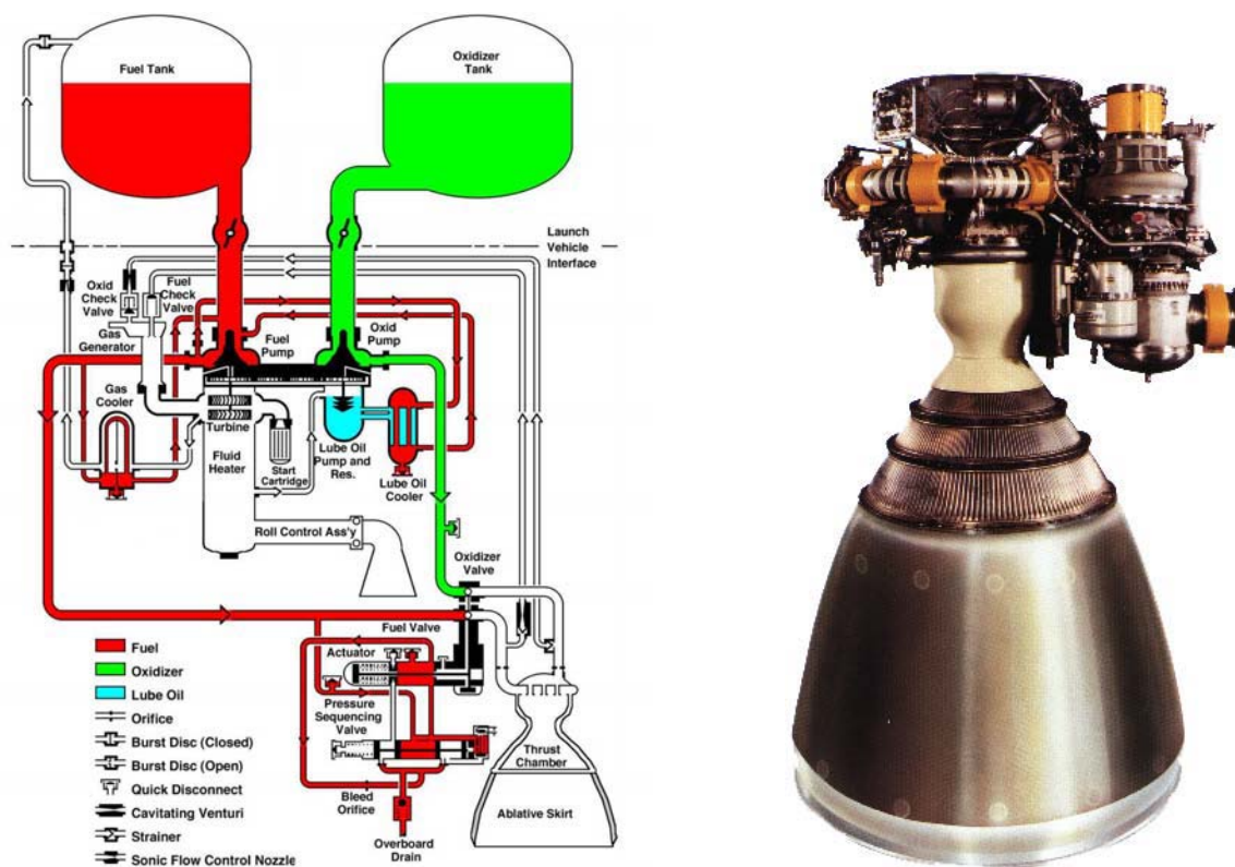
Figure 8.1-2. Titan IV Stage II LR91-AJ-11
