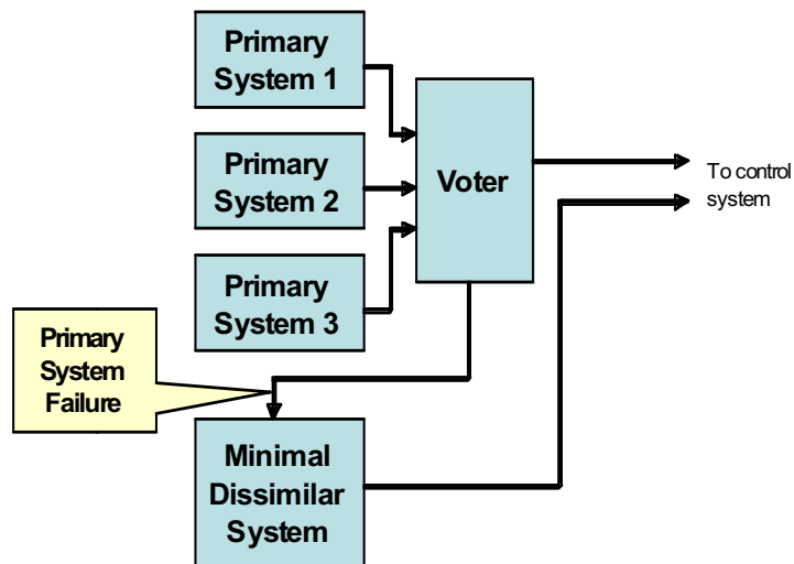
Figure 5.3-11. Triplicate system with dissimilar system
