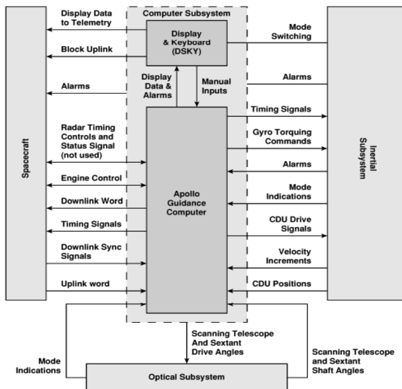
Figure 6.2-1. The Apollo Command Module and LEM GN&C Computer Architecture
