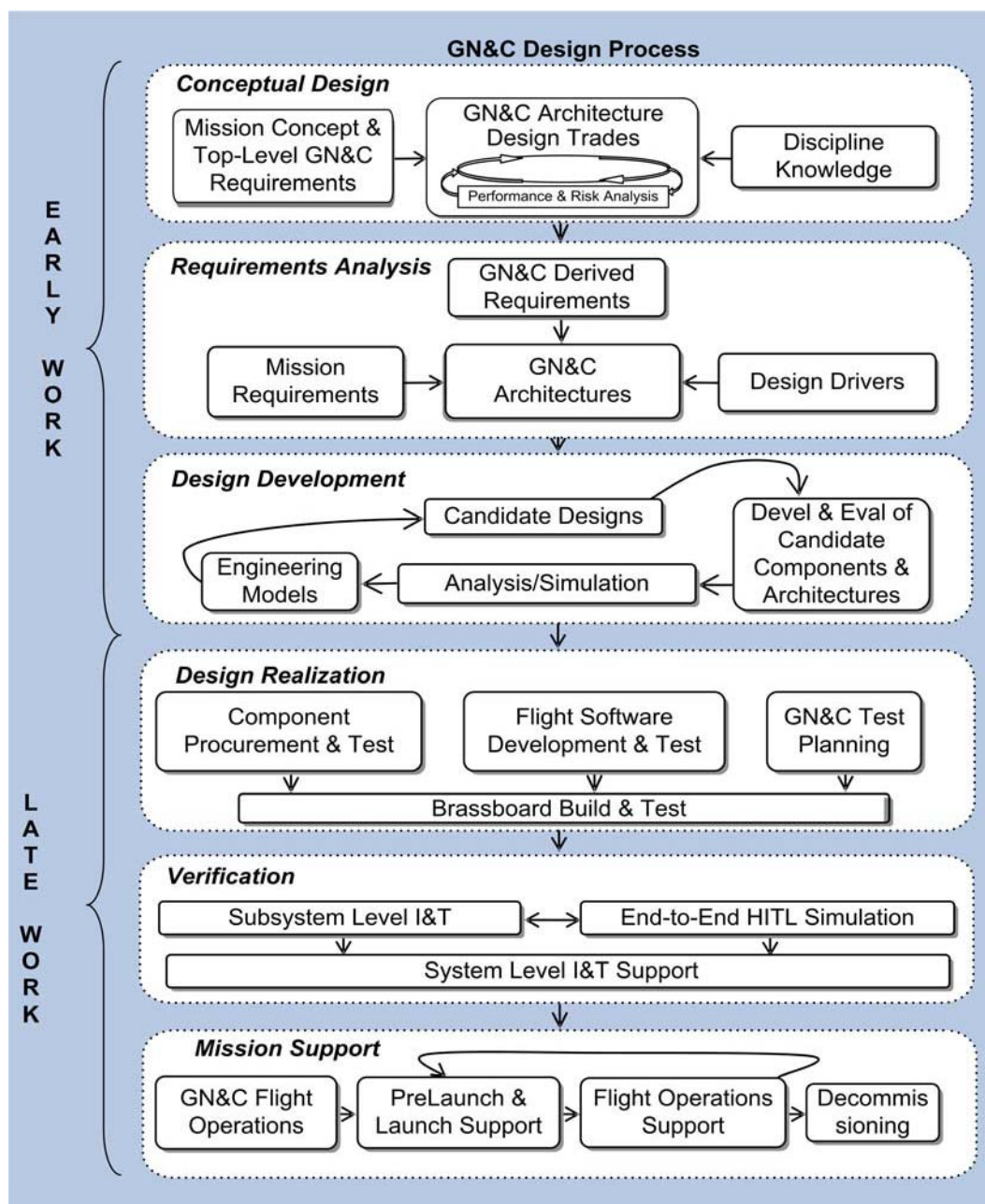
Figure 7.3-1. Overall GN&C DDT&E Process
