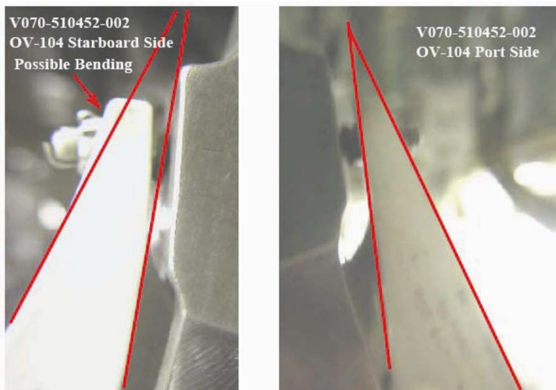
Figure 10.3-4. Comparison of Starboard and Port 452 Links [ref. 1]
