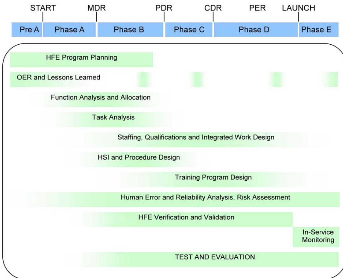
Figure 11.5-1. HFE Activities as Part of the Design Program
