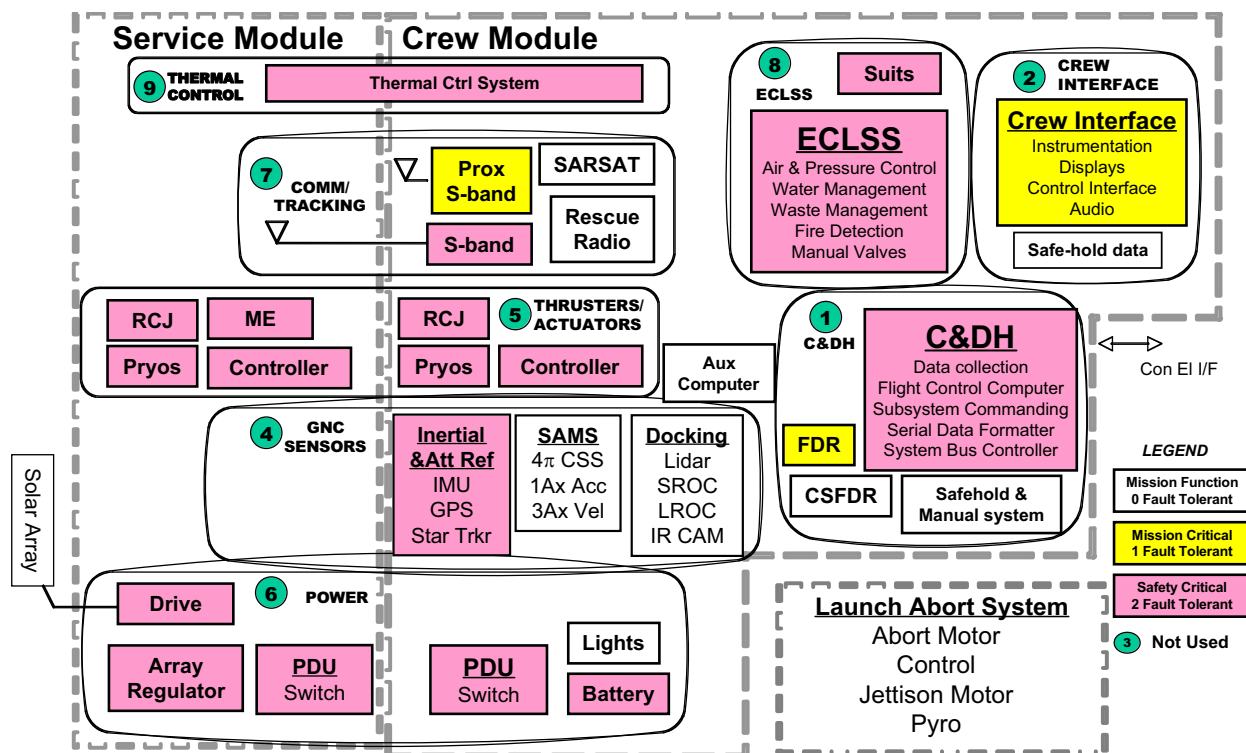
Figure 5.3-4. Notional Avionics Functional Block Diagram
