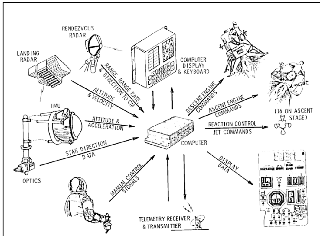
Figure A-4: APOLLO Lunar Module Guidance, Navigation, and Control
