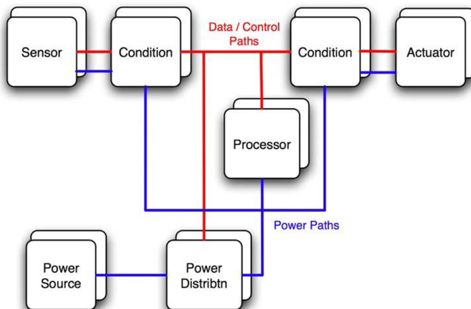
Figure 5.3-9. Notional Data / Control and Power Distribution Topology
