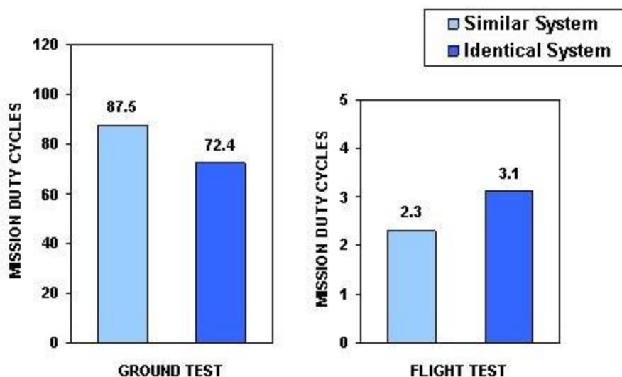
Figure 8.4-4. Apollo Service Propulsion System Testing Time [ref. 21]
