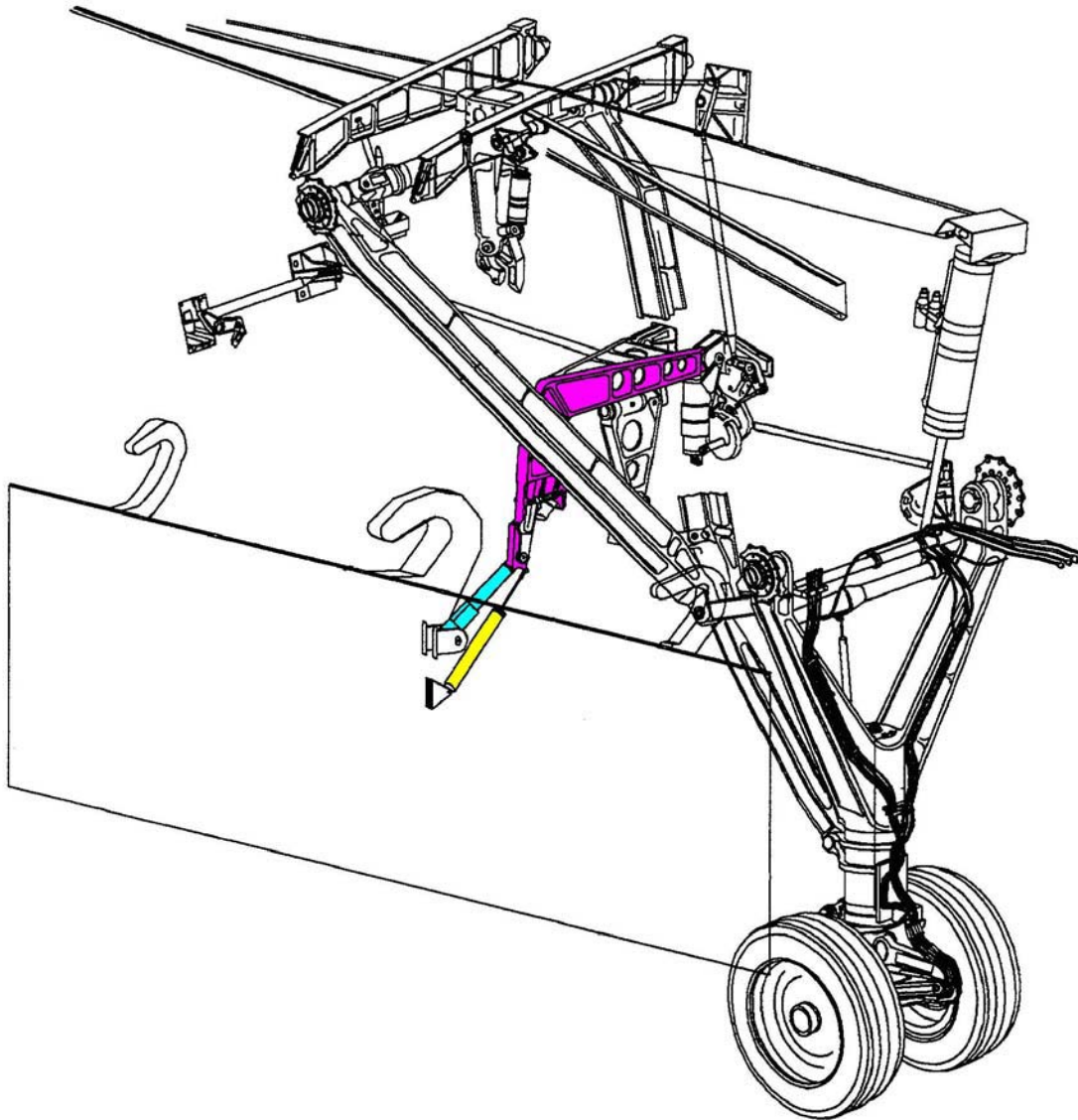
Figure 10.3-3. MLG Door Retract Mechanism [ref. ]
