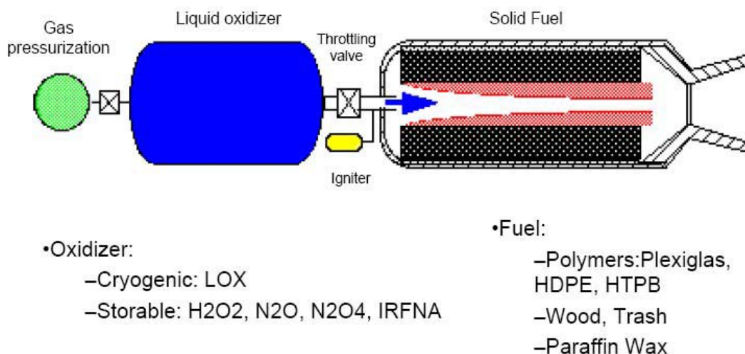
Figure 8.1-4. Simplified Hybrid Motor
