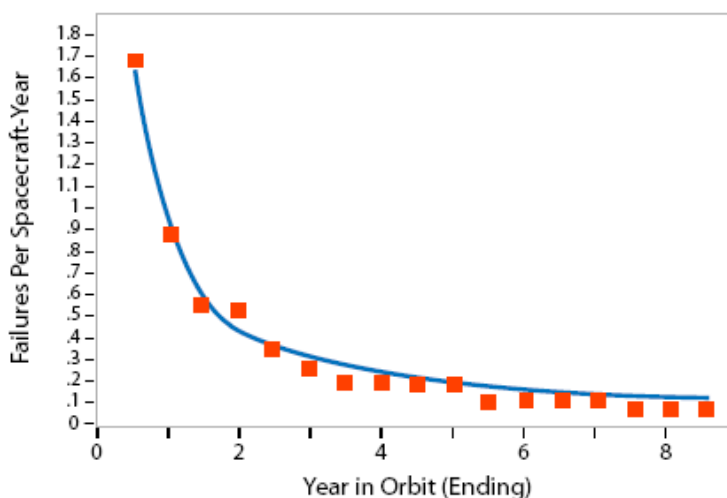
Figure 5.2-3. Trend of All Failures as a function of Time [ref. 17]
