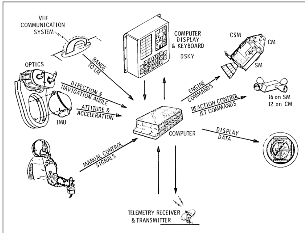
Figure A-3: APOLLO Command Module Guidance, Navigation, and Control.
