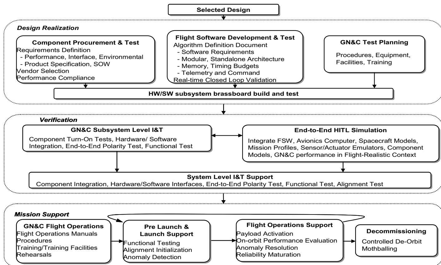
Figure 7.5-2. GN&C Design Process – Late Work
