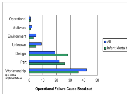
Figure 5.2-2. Orbital Experience from an Integration and Test Perspective [ref. 8]
