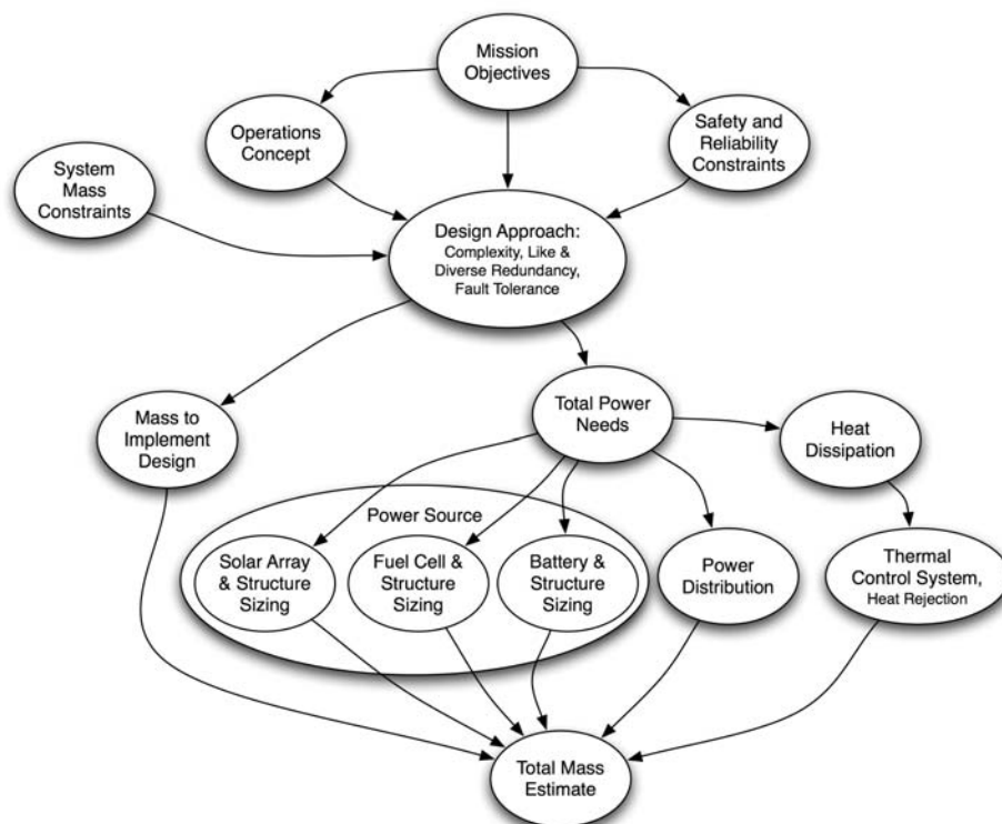
Figure 5.3-3. Power has a Multiplicative Influence on Mass Resources
