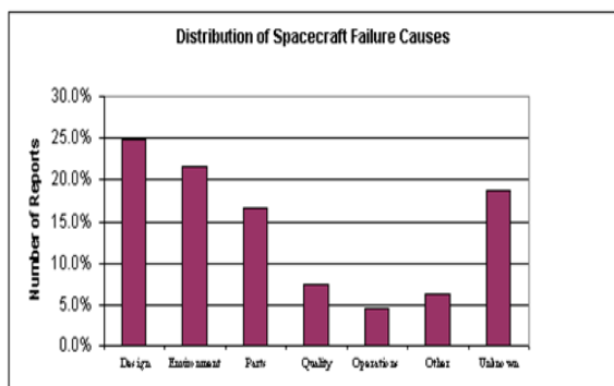
Figure 5.2-1. Distribution of Causes Reliability Prediction for Spacecraft, RADC-TR-85-229 [ref. 18]
