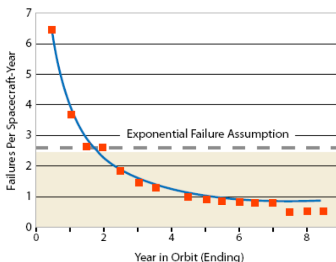
Figure 5.2-3. Trend of All Failures as a function of Time [ref. 17]
