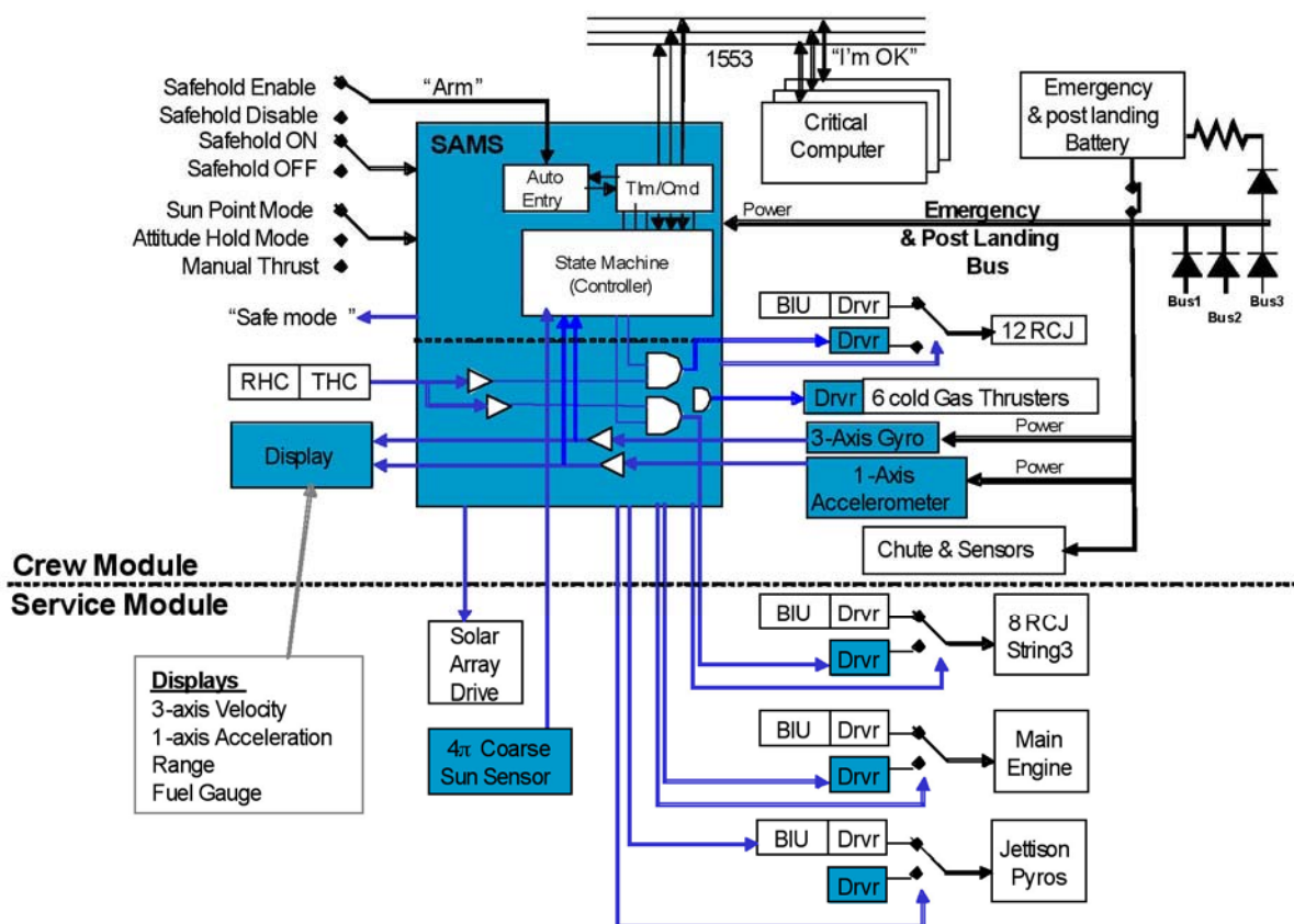
Figure 5.3-13. Notional Example of a Safe and Manual Mode Shown as Blue-Green Boxes
