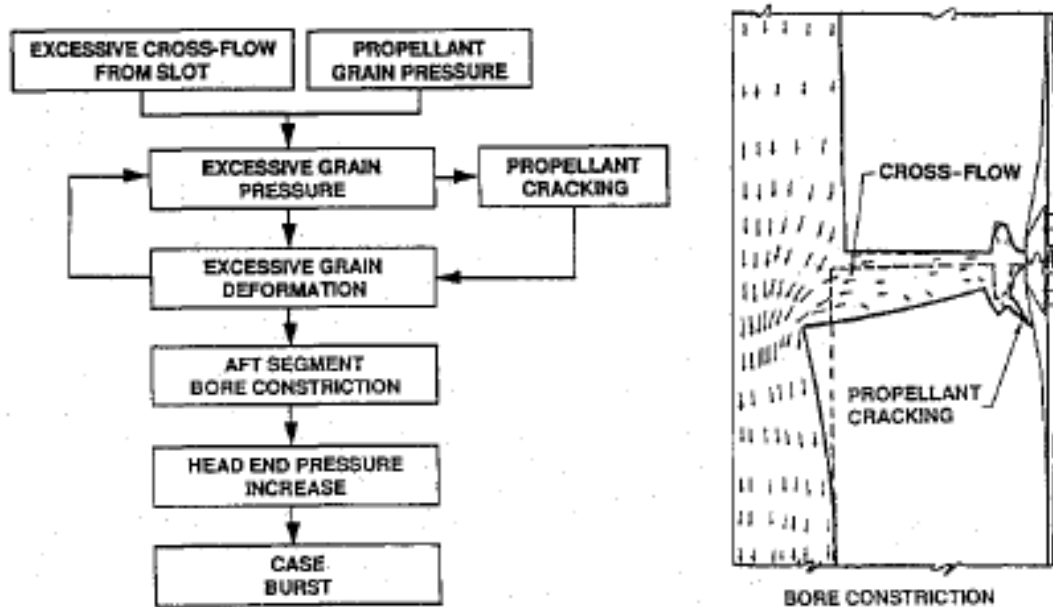
Figure 8.4-6. SRMU PQM-1 Test Failure Scenario [ref. 10]
