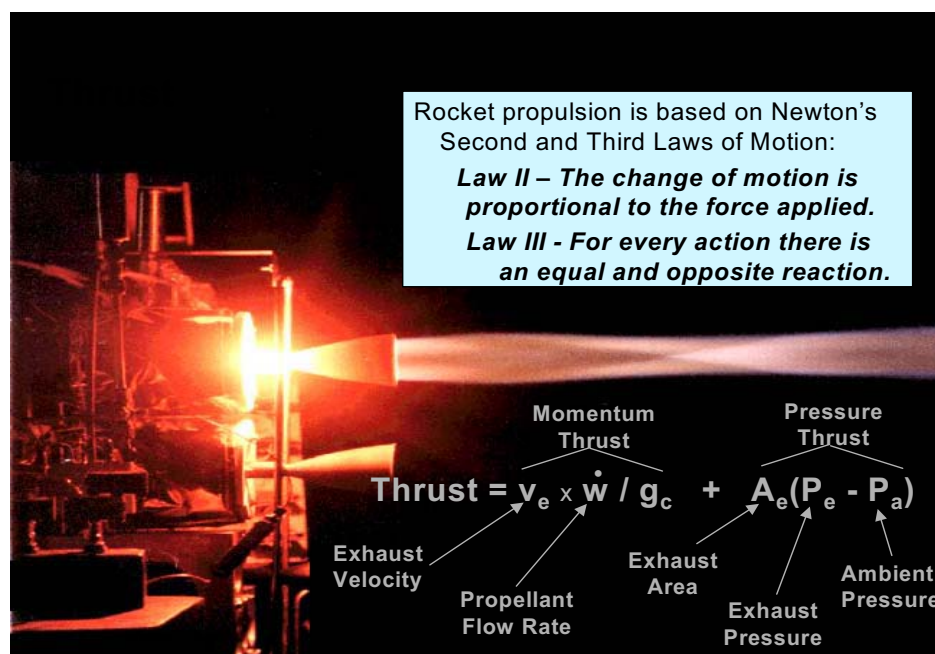
Figure 8.1-1. Propulsion System Basics
