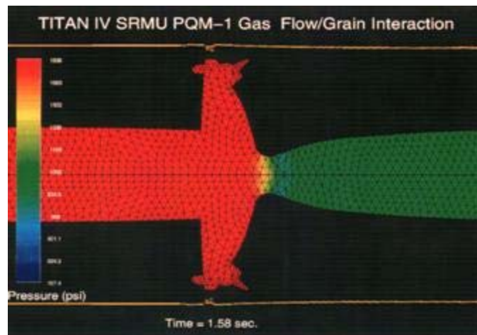
Figure 8.4-7. SRMU PQM-1 Computed Chamber Pressure 17
