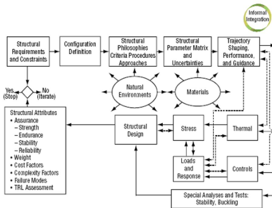
Figure 4.3-2. Structure Design Function Plane [ref. 9]
