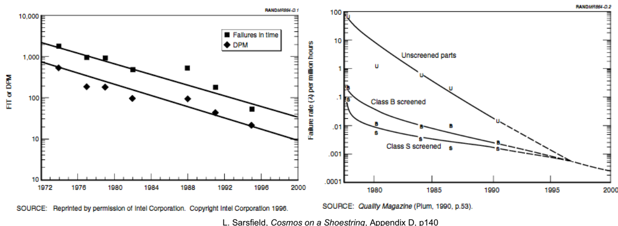
Figure 5.2-6. Progression of Semiconductor Parts Failure Rates
