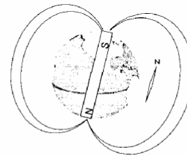
The Earth as a Magnet
