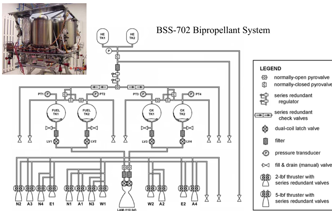
Figure 8.1-6. Space Propulsion System Schematic
