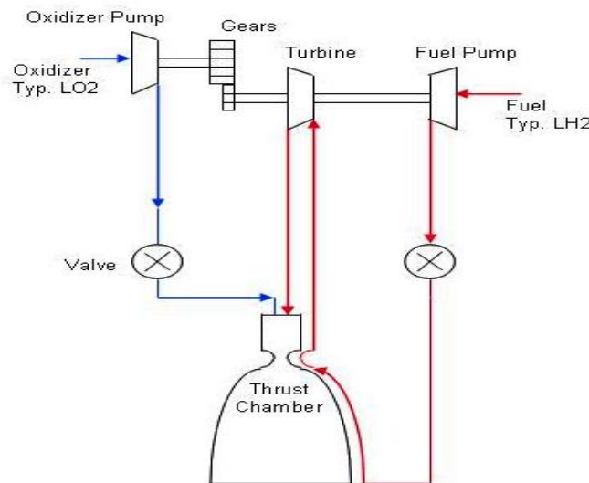
Figure 8.5-3. Expander Cycle 20 Engine or Motor Operating Pressure
