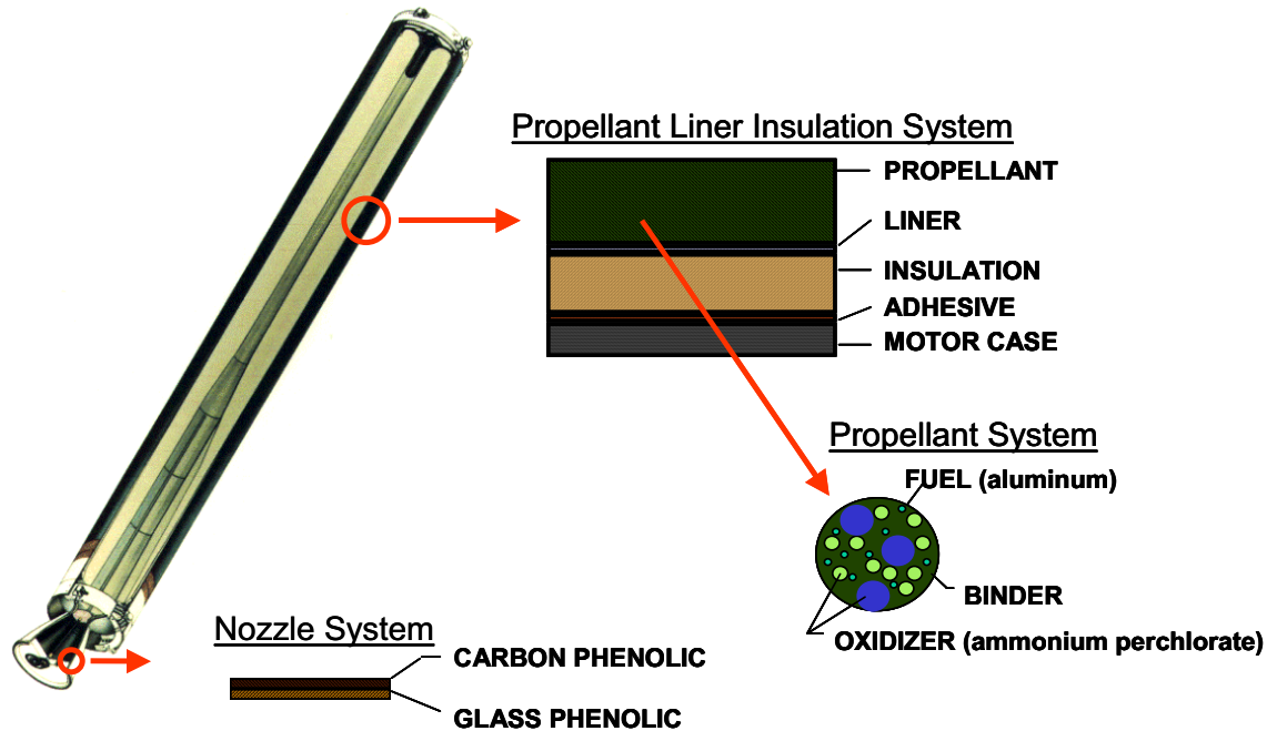
Figure 8.1-3. Delta II GEM 60 Solid Rocket Motor
