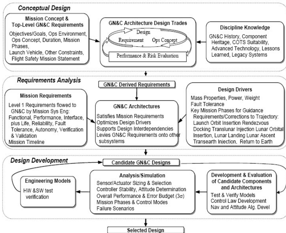
Figure 7.5-1. GN&C Design & Development Process – Late Work
