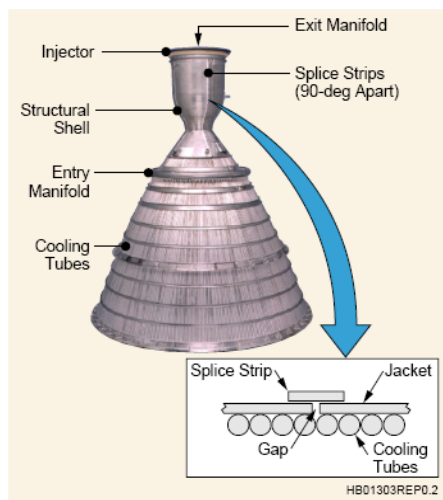
Figure 8.4-5. RL10B-2 Engine Combustion Chamber Construction [ref. 44]
