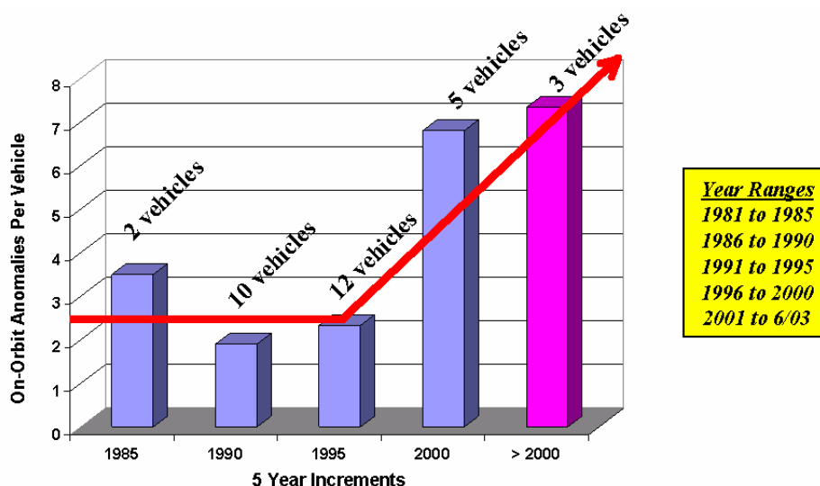
Figure 6.1-2. Trend of Software On-Orbit Software Anomalies
