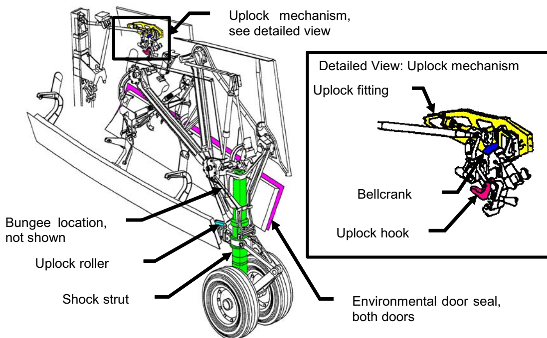
Figure 10.3-1. Nose Landing Gear Mechanisms [ref. 1]
