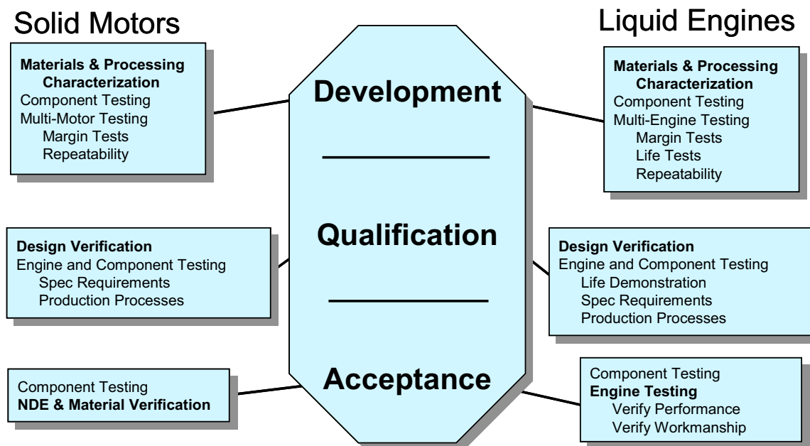
Figure 8.5-5. Propulsion System Testing
