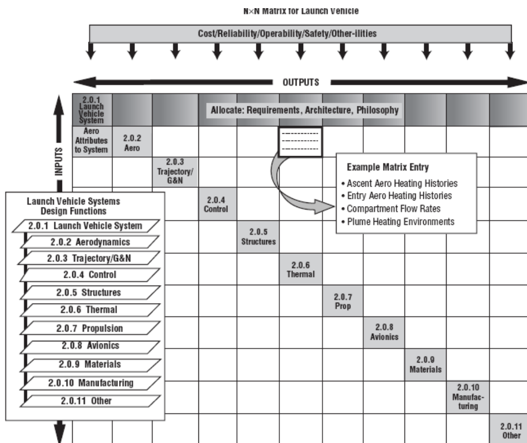
Figure 4.2-2. N x N Matrix Showing Possible Relationships Between Subsystems [ref. 9]
