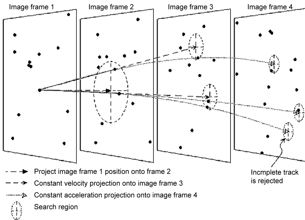
Figure 3.—Schematic illustration of how potentially valid tracks are identified. An empty search region terminates a track fragment. In this example, two valid tracks are identified for the original particle. The process is continued until only the valid track remains.
