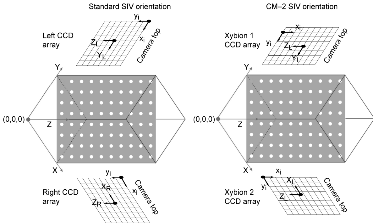
Figure 6.—SOFBALL camera orientation compared to standard SIV orientation. X, Y, Z: absolute coordinates. x_i, y_i : image coordinates. X_R, Z_R, Y_L, Z_L : window coordinates for right and left views.
