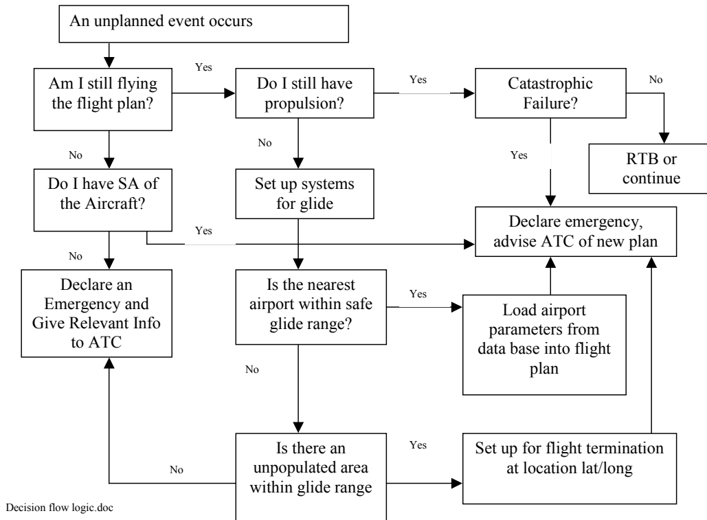
Figure 3.2.1-1. Normally the UAS Follows This Logic Sequence for Airborne Failures with a Functioning Data Link.
