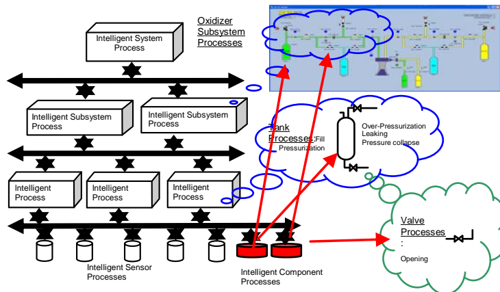
Figure 2. Encapsulation of process models at various levels of the architecture.
