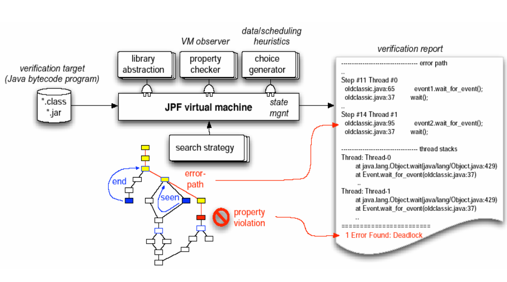
Figure 5 Java PathFinder Architecture
