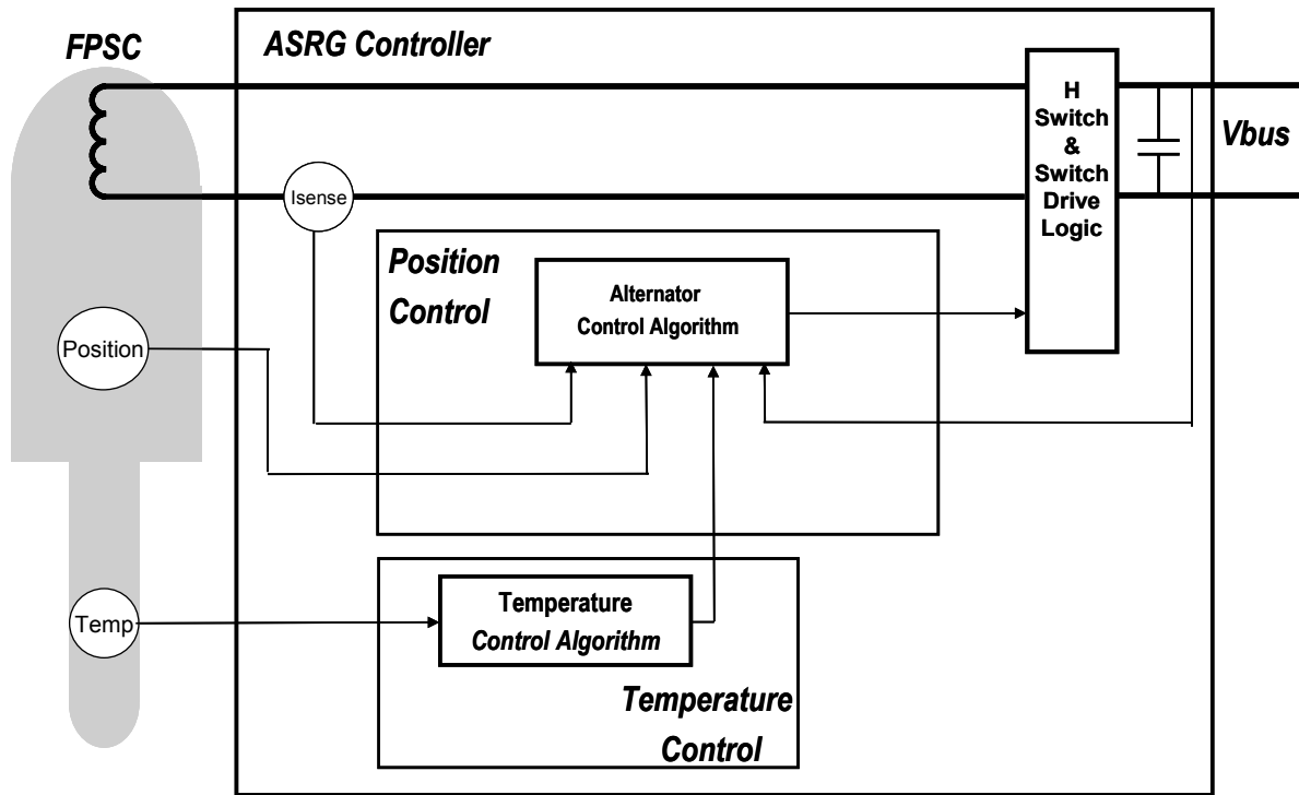
Figure 4.—ASRG algorithm block diagram.
