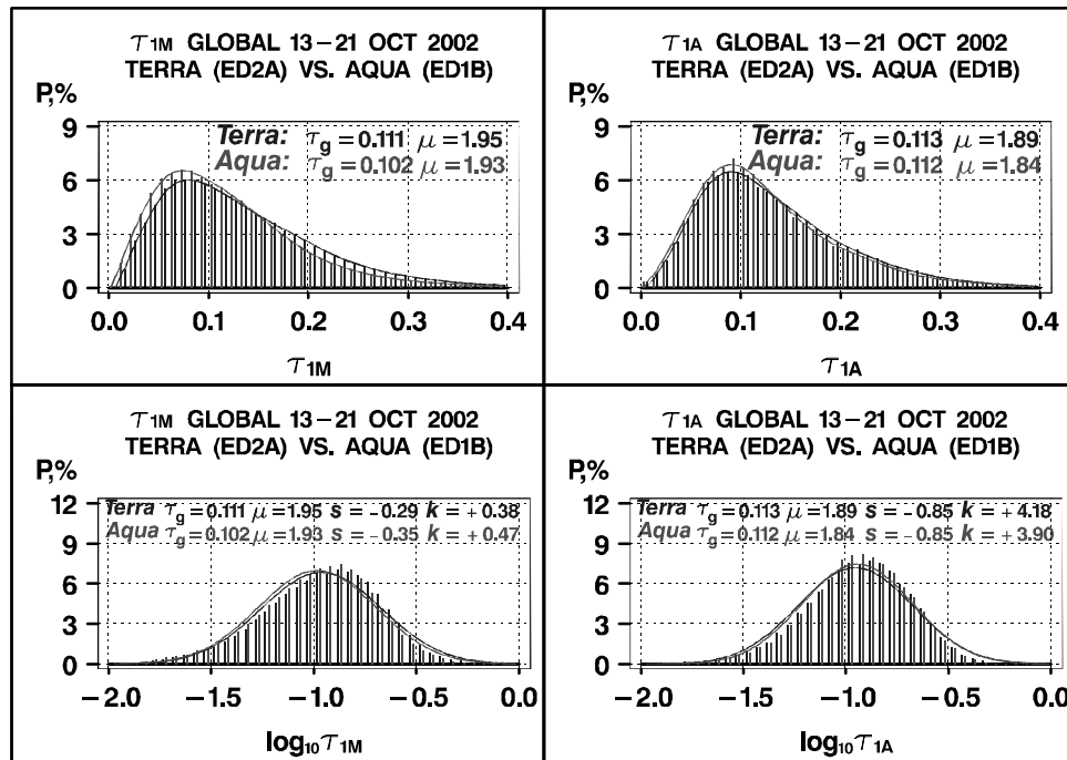
Figure 6. Top: Histograms of \tau_{1M} and \tau_{1A} derived from the current release CERES SSF ( 1^\circ ) 2 Terra (Edition 2A) and Aqua (Edition 1B) global data from 13-21 October 2002. Geometric mean and STD statistics are superimposed. Bottom: Same but for \log(\tau_{1M}) and \log(\tau_{1A}) . In addition to geometric mean and STD statistics, skewness ( s ) and kurtosis ( k ) are also shown. (Note that for a Gaussian distribution, s=k=0 .)
