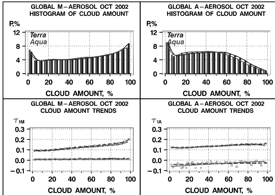
Figure 8. Same as in Fig. 3 but for the ambient cloud amount, A_T (binned at \Delta A_T=5\% ). Note that A_T was determined by the A-cloud screening. For the exact definition of A_T and for relevant discussion see section 4.1. In the M product, maximum of the A_T -histograms is found in the highest bin centered at A_T\sim 97.5\% (includes data with 95\leq A_T<100\% ), whereas in the A-product, it is in the lowest bin at A_T\sim 2.5\% (includes data with 0\leq A_T<5\% ). The average A_T is \sim 47\% in the M products compared to A_T\sim 32\% in the A-product (cf. data in Table 1). The \tau_{1A} -trends are smaller compared with \tau_{1M} trends, and more reproducible cross-platform. Small divergence between the two \tau_{1M} trends towards larger A_T 's may indicate residual cloud screening differences in the M product between the two platforms (cf. \tau_{1M}(N) trends in Fig. 3).
