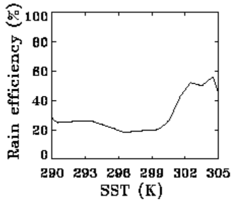
Fig. 16 DCS rainfall efficiency.
