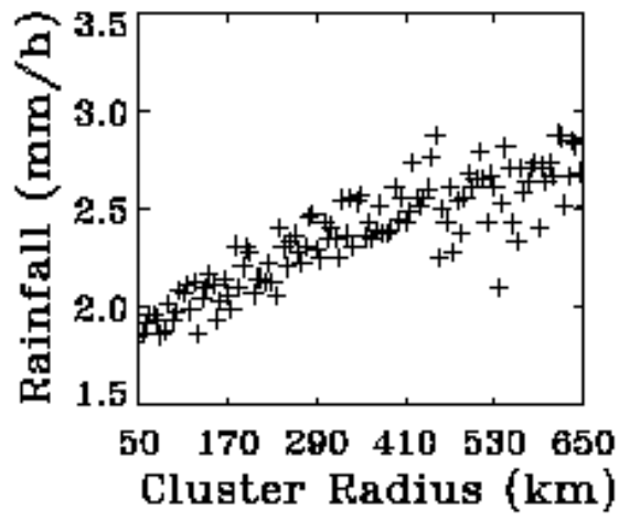
Fig. 4 The relationship between DCS effective size and rainfall rate.
