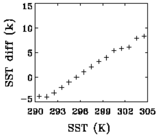
Fig. 12 Variations of SST difference on SST.
