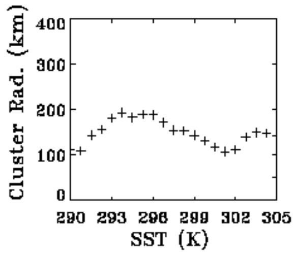
Fig. 2 DCS cluster effective size vs SST.
