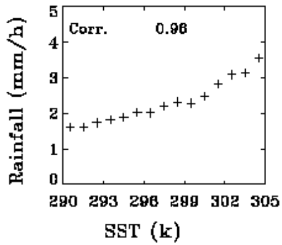
Fig. 3 Averaged DCS rainfall rates vs SST.
