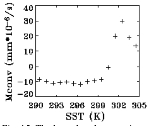
Fig. 15 The boundary layer moisture convergence.
