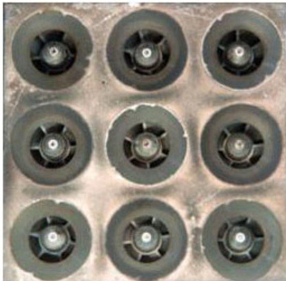
Figure 1.—Nine-element fuel injector module.
