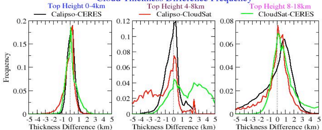
Figure 7: Cloud thickness frequency (top figure) and cloud thickness difference frequency of occurrence (bottom three figures) for single clouds over tropical ocean during daytime for April 2007.
