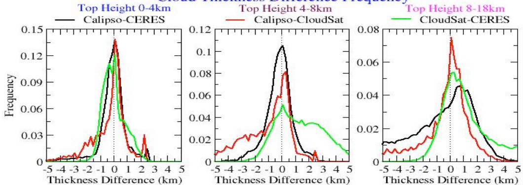
Figure 8: Same as Figure 7, except over land.
