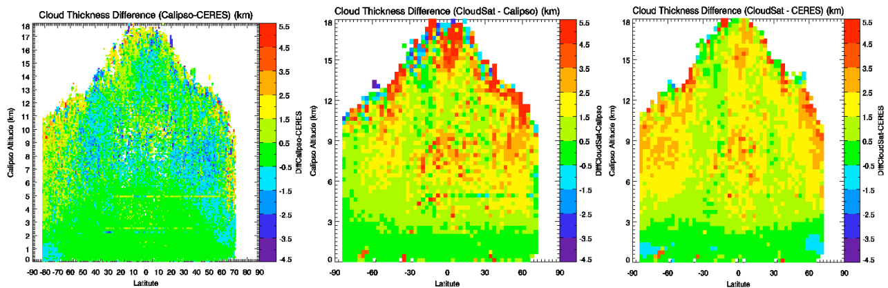
Figure 10: Zonal single layer cloud thickness difference densities among CALIPSO, CERES and CloudSat as functions of cloud altitude during daytime over ocean and land for April 2007. Left: CALIPSO-CERES, middle: CloudSat-CALIPSO, and right: CloudSat-CERES. Colors represent cloud thickness differences from -4.5 km (dark blue) to 5.5 km (red)
