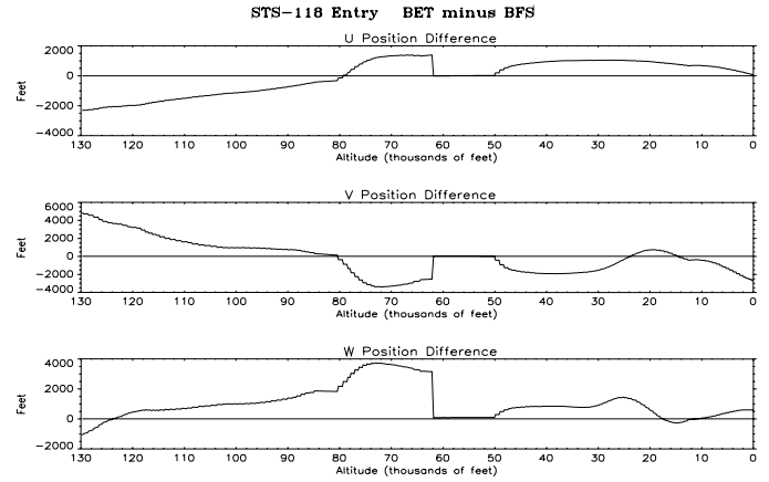
Fig. 15. STS-118 BET versus BFS position vector compare.
