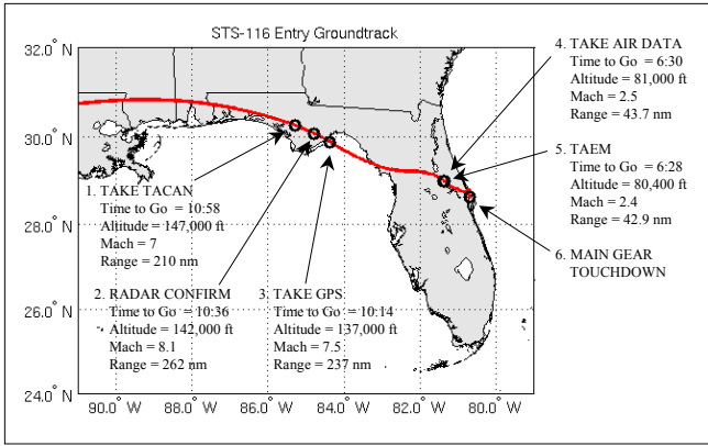
Fig. 5. STS-116 entry ground track.
