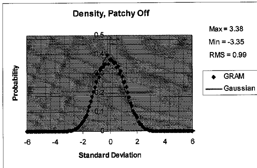
Figure 2. Comparison of Earth-GRAM07 density dispersions with a Gaussian distribution.
