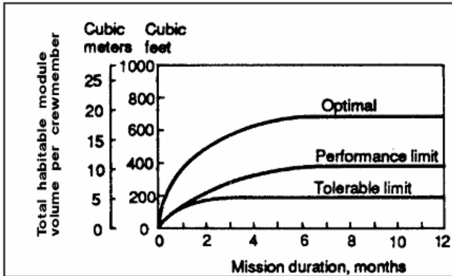
Figure 3. Habitable volume per crewmember as a function of mission duration & performance level. (NASA-STD-3000, 1995, Figure 8.6.2.1-1, from Celentano, Amorelli, & Freeman, 1963).
