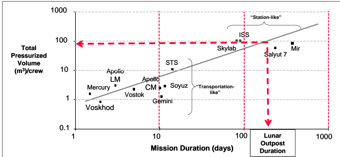
Figure 2. Total pressurized volume for “transportation-like” and “station-like” spacecraft as a function of mission duration.
