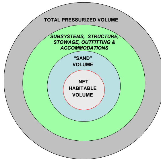
Figure 1. Spacecraft pressurized volumes conceptual relationships.
