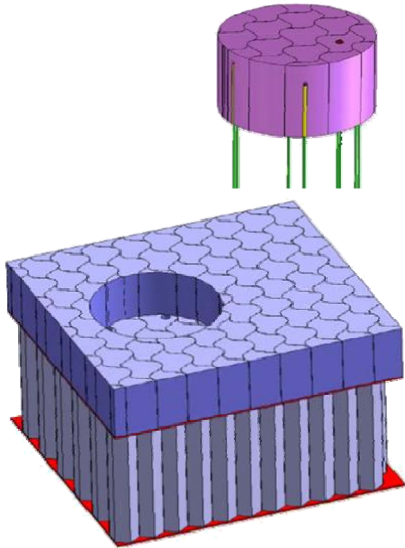
Figure 5. MISIP Plug and Acreage TPS/heatshield structure cavity.
