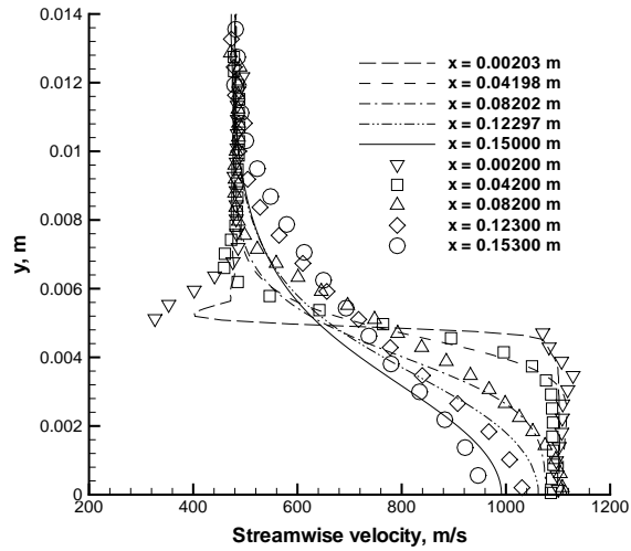
Figure 10: Comparison of RELIEF velocity data with simulation results
