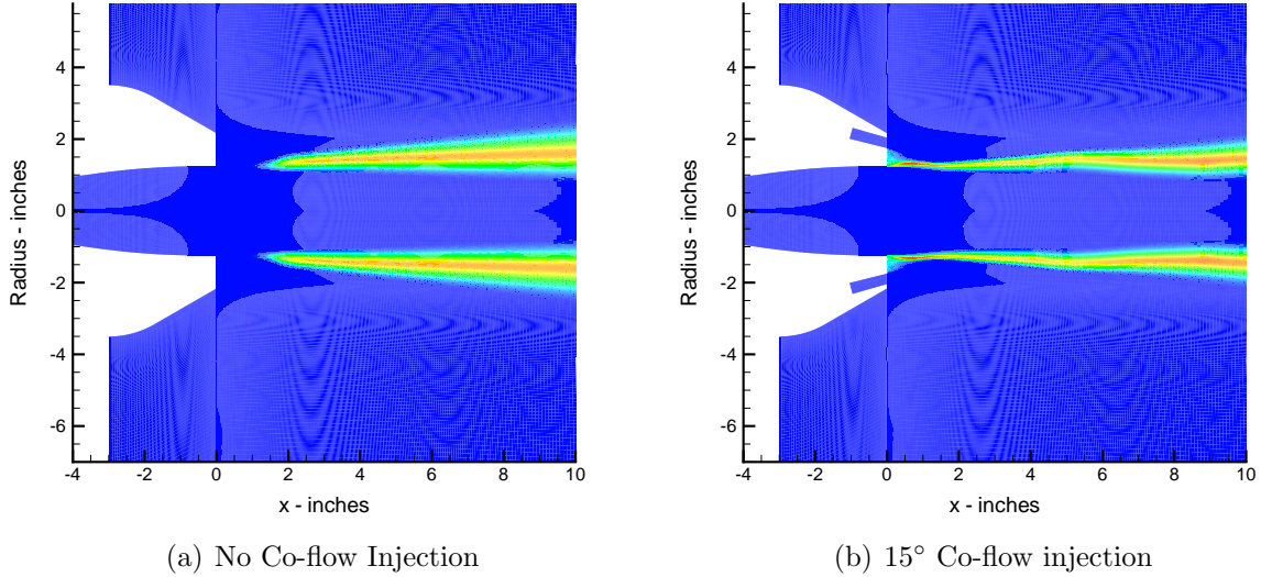
Figure 2: OH contours showing the sensitivity of the flame location to the presence of angled co-flow injection.
