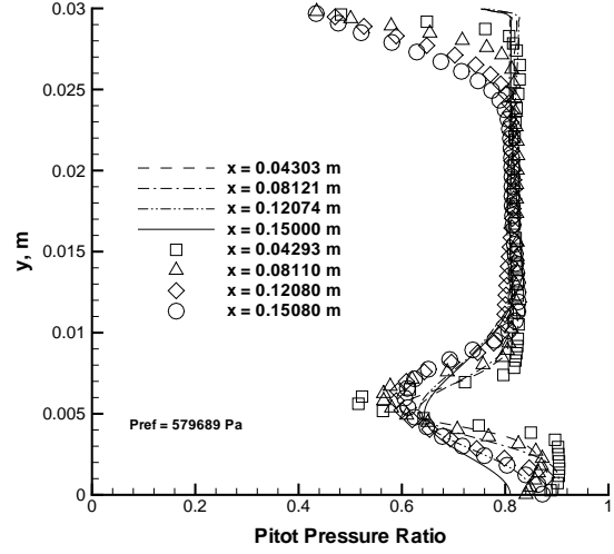
Figure 9: Comparison of pitot pressure data (symbols) with simulation results
