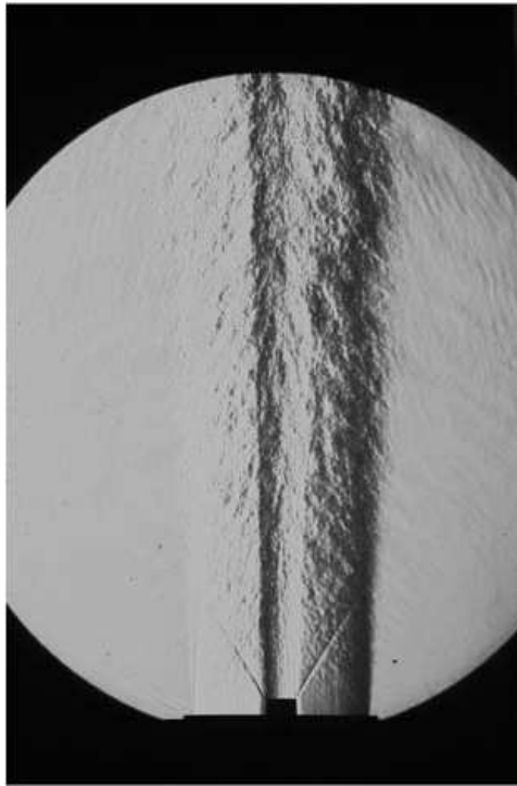
Figure 5: Schlieren image of coaxial jet mixing (conical extension cap removed)
