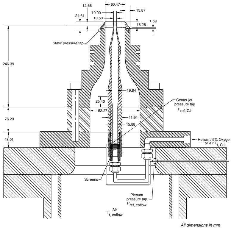
Figure 4: Coaxial jet assembly cross-section
