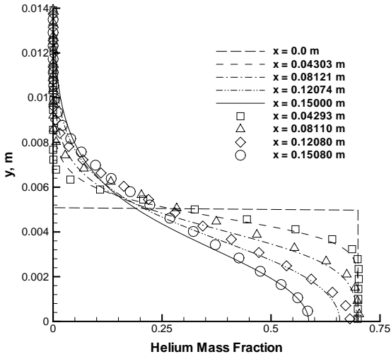
Figure 8: Comparison of helium mass fraction data (symbols) with simulation results
