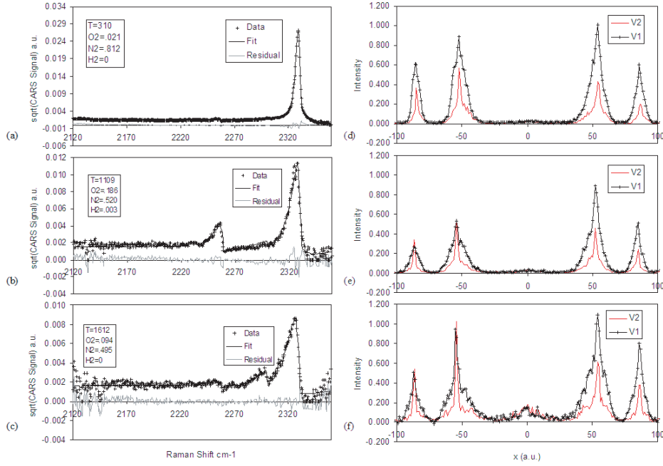
Figure 7: Simultaneous spectra of CARS (left) and Rayleigh scattering from two viewing directions (right). The CARS spectra are both data and fits of theory to the data. The Rayleigh spectra are data points connected by lines
