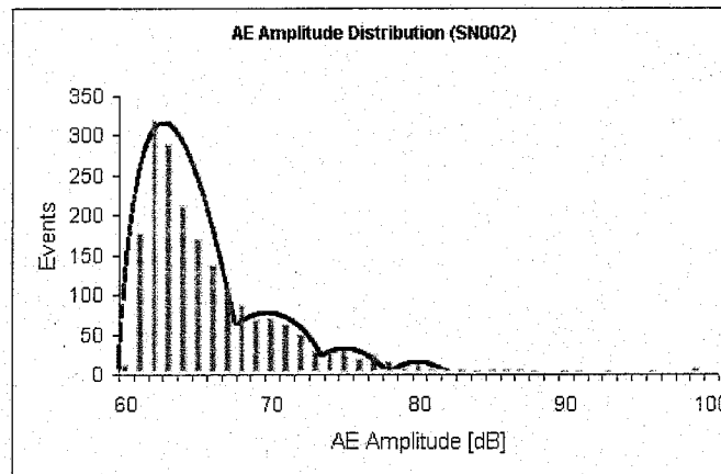
Figure 1 AE amplitude distribution for COPV SN002
