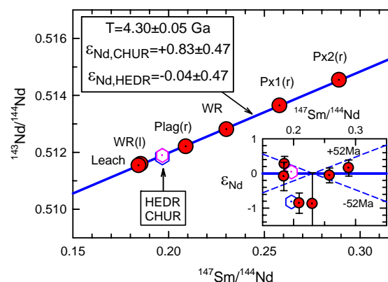
Figure 1. Sm-Nd data for Kalahari 009.
