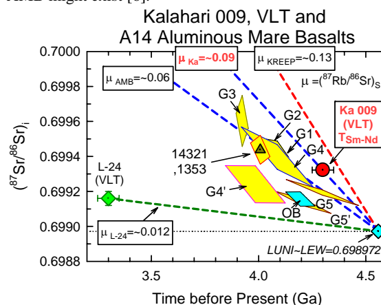
Figure 3. I(\text{Sr}) vs. T(\text{age}) of Kalahari 009 (red), L-24 VLT (green) and various groups of A14 AMBs (yellow).
