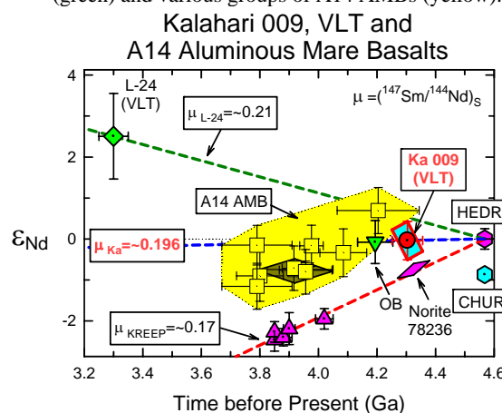
Figure 4. \epsilon_{\text{Nd}} vs. T(\text{age}) of Kalahari 009 (red), L-24 VLT (green) and A14 aluminous mare basalts (yellow).
