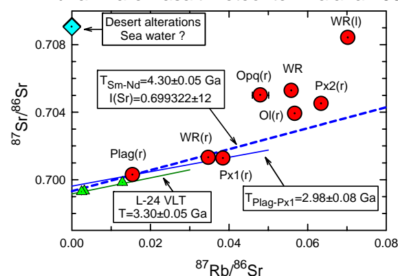
Figure 2. Rb-Sr data for Kalahari 009.
