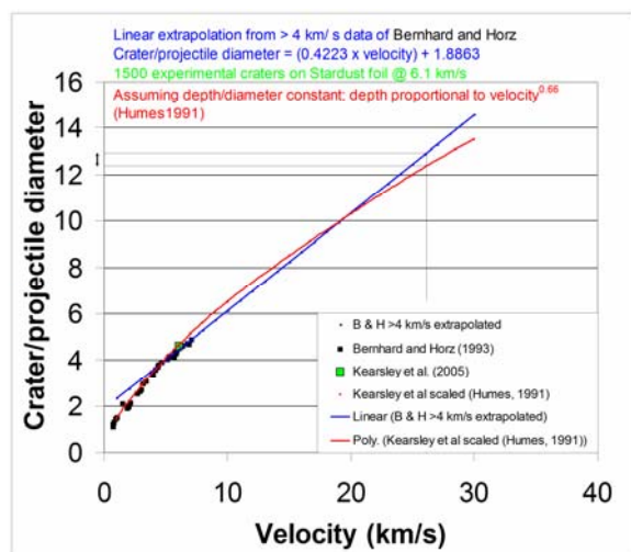
Figure 1. Extrapolation of existing crater size calibration data. Experimental data is still needed for 10-30 \text{km s}^{-1} range to bracket Stardust ISP collection velocity. Raw data plotted is extracted from [7], and Stardust foil craters [8] scaled by relationship described in [9].
