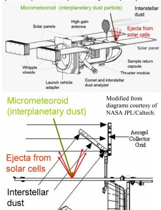
Figure 2. Possible impacts on the aft solar panels.
