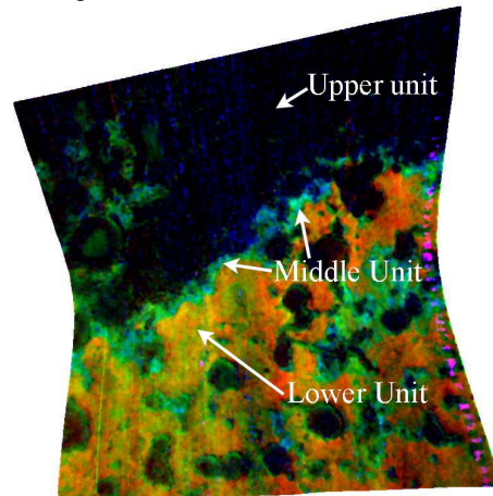
Figure 3: (B) Color composite of parameter maps for FRT8838, where R: D2300 (2.3 \mu\text{m} feature [7]), G: OLINDEX (ferrous index), B: BD2210 (2.21 \mu\text{m} feature).
