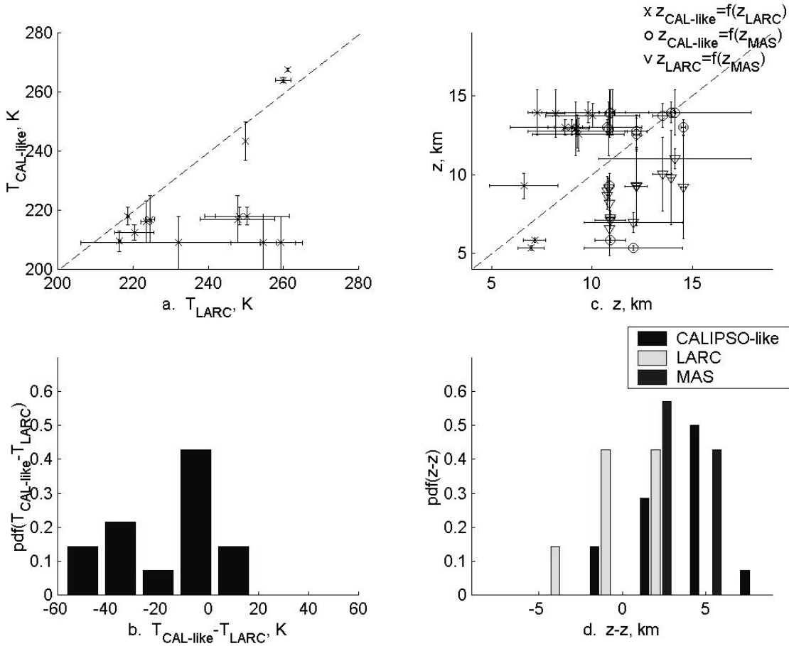
Figure 10: CRYSTAL-FACE cloud cases (a) T_{CAL-like} = f(T_{LaRC}) , (b) probability density function of T_{CAL-like} - T_{LaRC} , (c) z_{CAL-like} = f(z_{LaRC}) in X, z_{CAL-like} = f(z_{MAS}) in O, z_{LaRC} = f(z_{MAS}) in V, (d) probability density function of z_{CAL-like} - z_{LaRC} , probability density function of z_{CAL-like} - z_{MAS} , probability density function of z_{LaRC} - z_{MAS} . Dashed lines are x = y .
