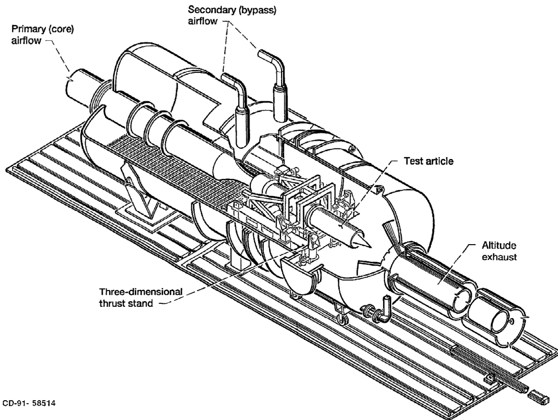
Figure 7.—Advanced nozzle test facility (CE-22).
