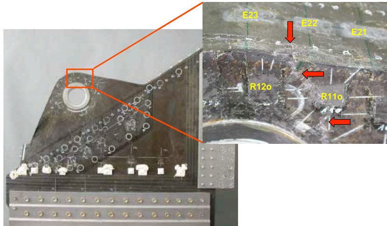
Figure 23. 2003-Subcomponent Test – Observed Failure (Red arrows point to the primary fracture path). that observed during the SC test shown in Figure 23. This damage is consistent with the damage seen in the other cases.
