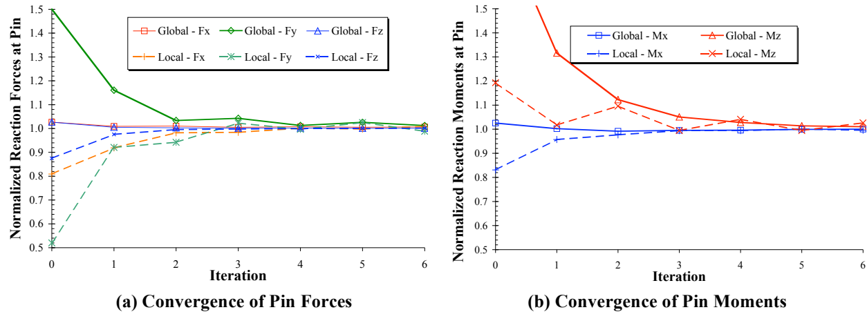
Figure 14. Convergence in Global-Local Analysis (Load Case W375).
