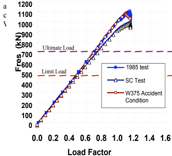
Figure 27. F_{Res} vs. Load Factor Variation for 1985-Certification Test, 2003-Subcomponent Test, and W375 Accident Case.
