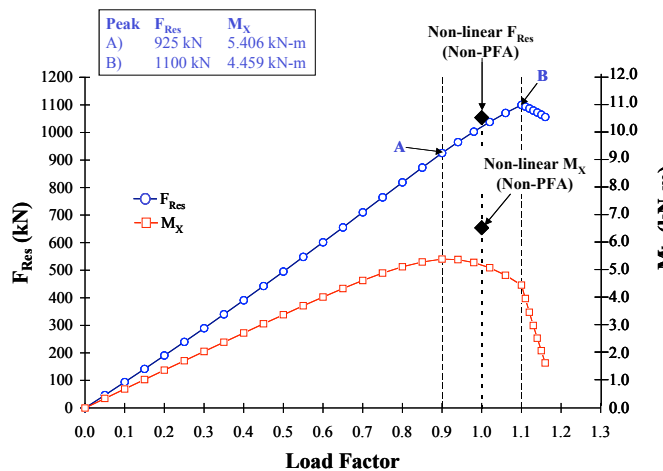
Figure 24. Load and Moment vs. Load Factor for W375 Load Case.
