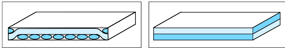
Figure 6. Eight-Harness Satin Weave and Tape Approximation.
