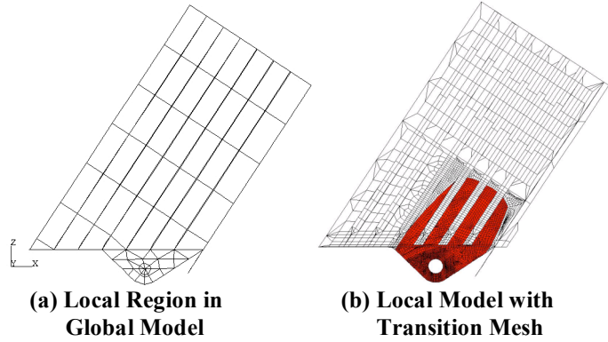
Figure 11. Models of Region Near Right Rear Lug.
