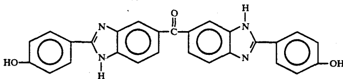
b) 5,5'-Carbonyl-bis[2-(4-hydroxyphenyl)benzimidazole]
