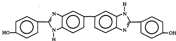
a) 5,5'-Bis[2-(4-hydroxyphenyl)benzimidazole]
