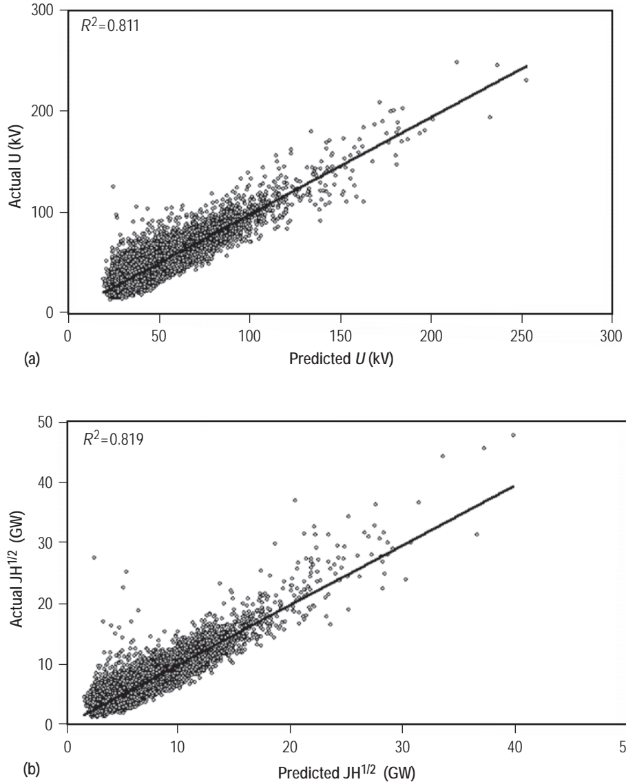
Figure 17. Correlation of the actual (AMIE) and predicted hourly mean values of the CPC voltage ( U ) and JH^{1/2} for all days of 1998. This shows extremely high correlation ( R^2 \approx 0.81-0.82 ) for both U voltage and JH^{1/2} (data courtesy of Aaron Ridley, University of Michigan).
