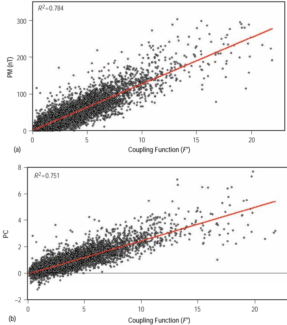
Figure 6. Correlation between (a) the PM index and coupling function ( F^* ) and (b) the PC index and coupling function ( F^* ) for 1997—related to low solar activity.
