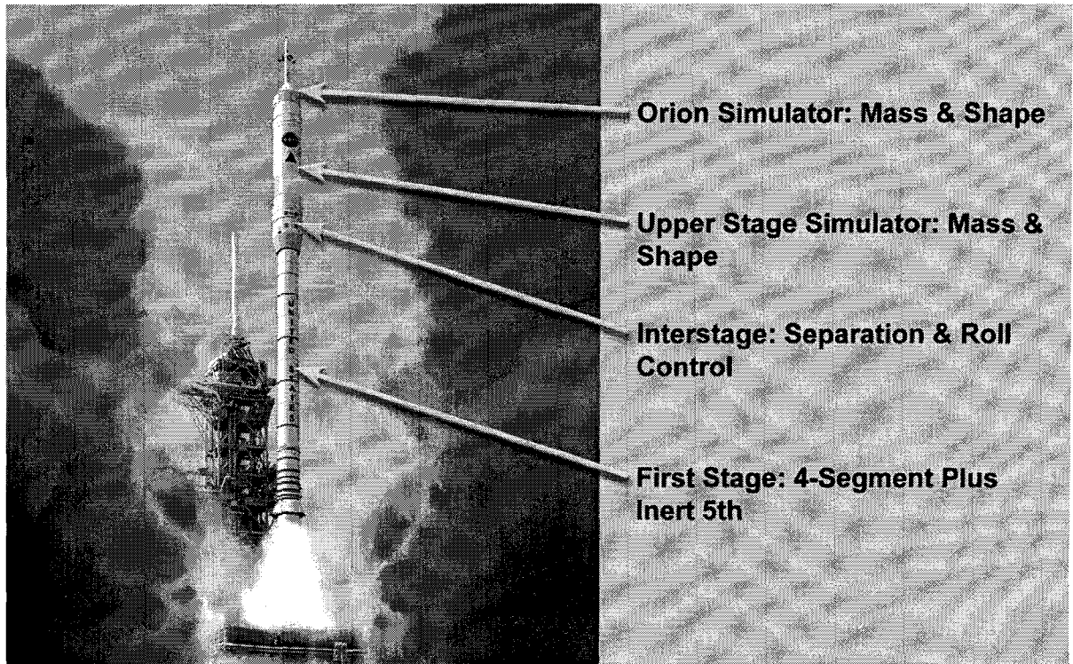
Figure 4. The Ares I flight test is planned for April 2009.
