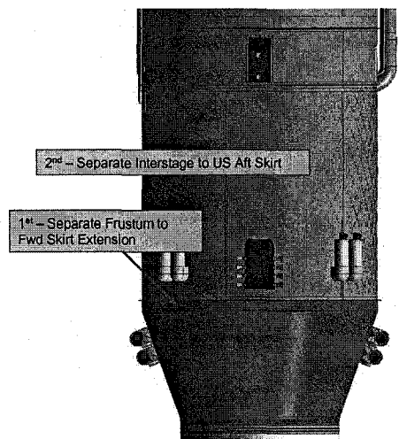
Figure 10. Locations of separation planes.
