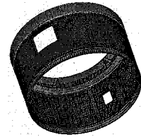
Figure 7. Computerized representation of forward skirt.
