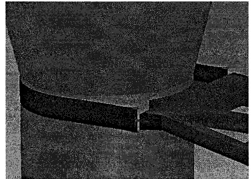
Figure 8. Conceptual design for wrap-around hold-down system to be used for on-pad stability.
