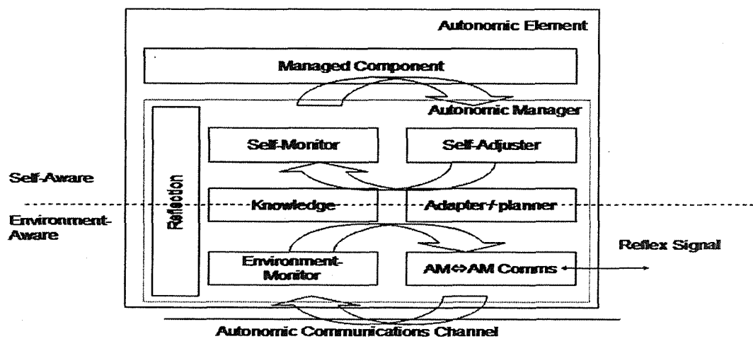
Figure 2: Autonomic Element, with reflection and reflex layers.
