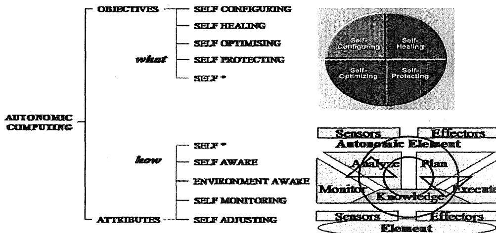
Figure 1: Properties of an Autonomic Computing System.
