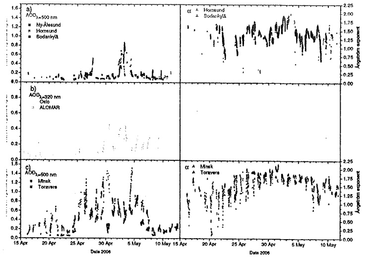
Figure 4: Left column: Aerosol optical depth for (a) Ny-Ålesund, Hornsund and, Sodankylä, (b) ALOMAR and Oslo (c) Minsk, Toravere. Right column: Angstrom exponent for Hornsund and, Sodankylä in the upper panel and for Toravere and Minsk in the lower panel.
