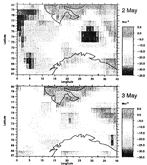
Figure 9: Radiative forcing of the episode relative to an aerosol situation in the spring with AOD=0.05.
