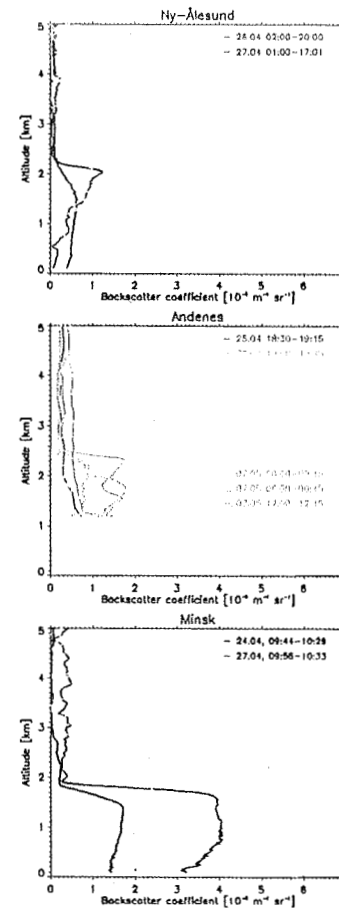
Figure 8: Height profiles of backscatter coefficients of aerosols from ground based observations at the sites in Ny-Ålesund, Andenes (ALOMAR), and Minsk during spring 2006
